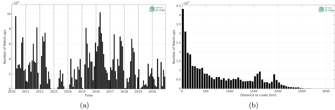
Figure 1: Number of match-ups between TSG (SAMOS) and SMOS SSS L3 v5 - 18 Days (CATDS-CECOS-LOCEAN) SSS as a function of time (a) and as function of the distance to coast (b) over the Tropical Pacific Ocean Pi-MEP region and for the full satellite product period.
