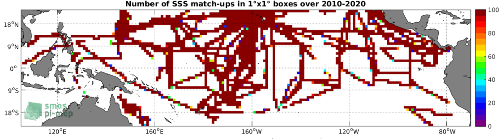
Figure 4: Number of SSS match-ups between TSG (SAMOS) SSS and the SMOS SSS L3 v5 - 18 Days (CATDS-CECOS-LOCEAN) SSS product for the Tropical Pacific Ocean Pi-MEP region over 1^\circ \times 1^\circ boxes and for the full satellite product period.
