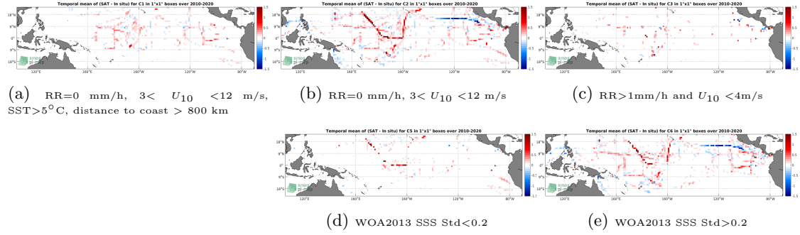
Figure 12: Temporal mean gridded over spatial boxes of size 1^{\circ} \times 1^{\circ} of \Delta\text{SSS} (SMOS SSS L3 v5 - 18 Days (CATDS-CECOS-LOCEAN) - TSG (SAMOS)) for 5 different subdatasets corresponding to:RR=0 mm/h, 3 < U_{10} < 12 m/s, SST >5^{\circ}\text{C} , distance to coast > 800 km (a), RR=0 mm/h, 3 < U_{10} < 12 m/s (b), RR >1 mm/h and U_{10} < 4 m/s (c), WOA2013 SSS Std <0.2 (d), WOA2013 SSS Std >0.2 (e).
