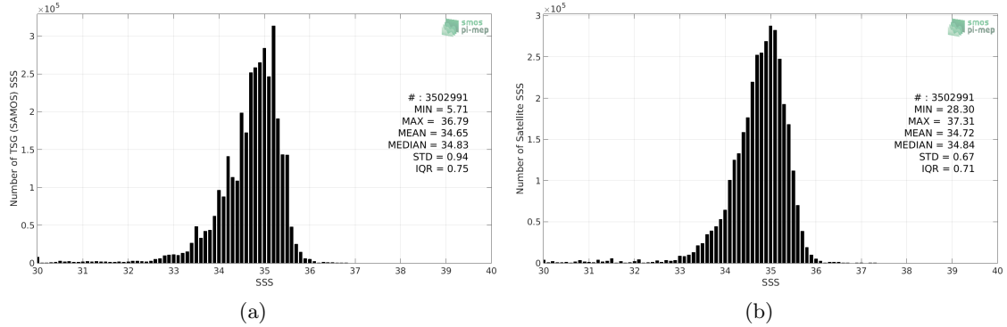
Figure 2: Histograms of SSS from TSG (SAMOS) (a) and SMOS SSS L3 v5 - 18 Days (CATDS-CECOS-LOCEAN) (b) considering all match-up pairs per bins of 0.1 over the Tropical Pacific Ocean Pi-MEP region and for the full satellite product period.
