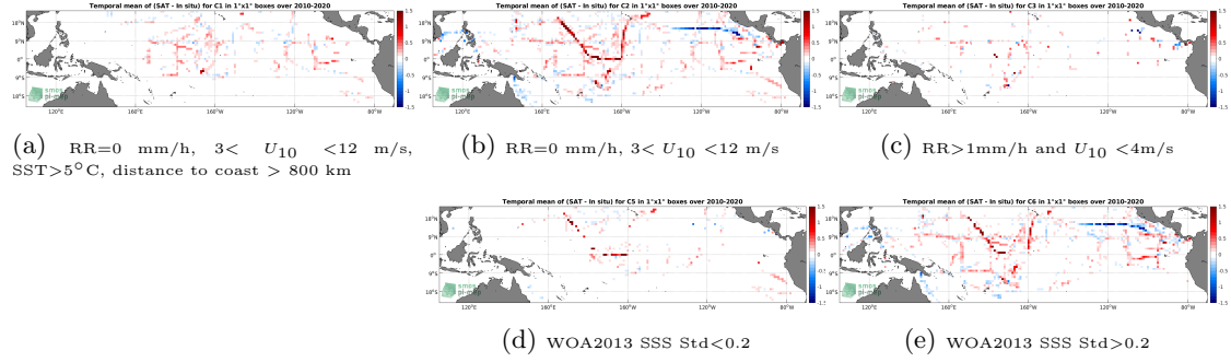
Figure 12: Temporal mean gridded over spatial boxes of size 1^{\circ}\times 1^{\circ} of \Delta\text{SSS} (SMOS SSS L3 v5 - 18 Days (CATDS-CECOS-LOCEAN) - TSG (SAMOS)) for 5 different subdatasets corresponding to:RR=0 mm/h, 3 < U_{10} < 12 m/s, SST >5^{\circ}\text{C} , distance to coast > 800 km (a), RR=0 mm/h, 3 < U_{10} < 12 m/s (b), RR >1 mm/h and U_{10} < 4 m/s (c), WOA2013 SSS Std <0.2 (d), WOA2013 SSS Std >0.2 (e).
