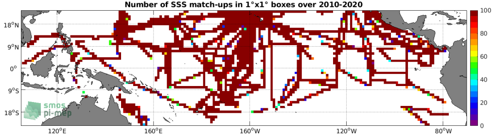
Figure 4: Number of SSS match-ups between TSG (SAMOS) SSS and the SMOS SSS L3 v5 - 18 Days (CATDS-CECOS-LOCEAN) SSS product for the Tropical Pacific Ocean Pi-MEP region over 1^\circ \times 1^\circ boxes and for the full satellite product period.
