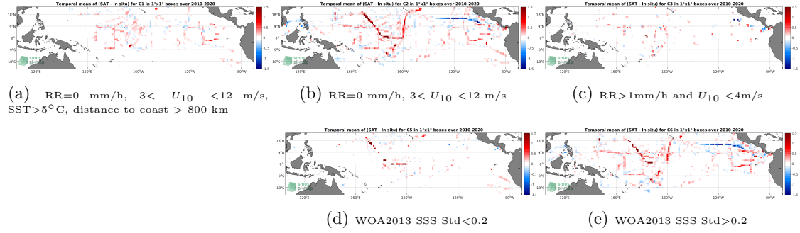
Figure 12: Temporal mean gridded over spatial boxes of size 1^{\circ}\times 1^{\circ} of \Delta\text{SSS} (SMOS SSS L3 v5 - 18 Days (CATDS-CECOS-LOCEAN) - TSG (SAMOS)) for 5 different subdatasets corresponding to:RR=0 mm/h, 3 < U_{10} < 12 m/s, SST >5^{\circ}\text{C} , distance to coast > 800 km (a), RR=0 mm/h, 3 < U_{10} < 12 m/s (b), RR >1 mm/h and U_{10} < 4 m/s (c), WOA2013 SSS Std <0.2 (d), WOA2013 SSS Std >0.2 (e).
