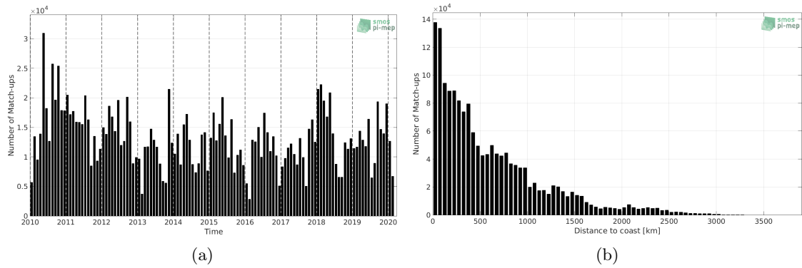
Figure 1: Number of match-ups between TSG (LEGOS-DM) and SMOS SSS L3 v5 - 18 Days (CATDS-CECOS-LOCEAN) SSS as a function of time (a) and as function of the distance to coast (b) over the Tropical Pacific Ocean Pi-MEP region and for the full satellite product period.
