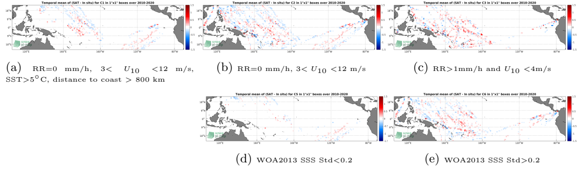
Figure 12: Temporal mean gridded over spatial boxes of size 1^{\circ}\times 1^{\circ} of \Delta\text{SSS} (SMOS SSS L3 v5 - 18 Days (CATDS-CECOS-LOCEAN) - TSG (LEGOS-DM)) for 5 different subdatasets corresponding to:RR=0 mm/h, 3 < U_{10} < 12 m/s, SST >5^{\circ}\text{C} , distance to coast > 800 km (a), RR=0 mm/h, 3 < U_{10} < 12 m/s (b), RR >1\text{mm/h} and U_{10} < 4\text{m/s} (c), WOA2013 SSS Std <0.2 (d), WOA2013 SSS Std >0.2 (e).
