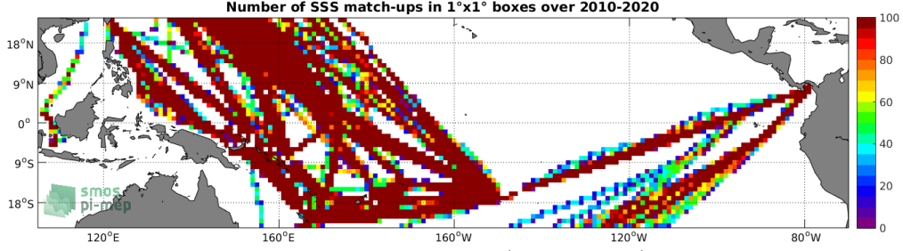
Figure 4: Number of SSS match-ups between TSG (LEGOS-DM) SSS and the SMOS SSS L3 v5 - 18 Days (CATDS-CECOS-LOCEAN) SSS product for the Tropical Pacific Ocean Pi-MEP region over 1^\circ \times 1^\circ boxes and for the full satellite product period.
