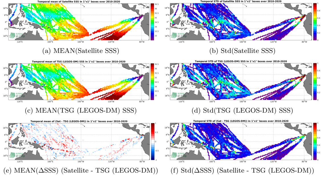
Figure 6: Temporal mean (left) and Std (right) of SSS from SMOS SSS L3 v5 - 18 Days (CATDS-CECOS-LOCEAN) (top), TSG (LEGOS-DM) (middle), and of \Delta SSS (Satellite - TSG (LEGOS-DM)). Only match-up pairs are used to generate these maps.
