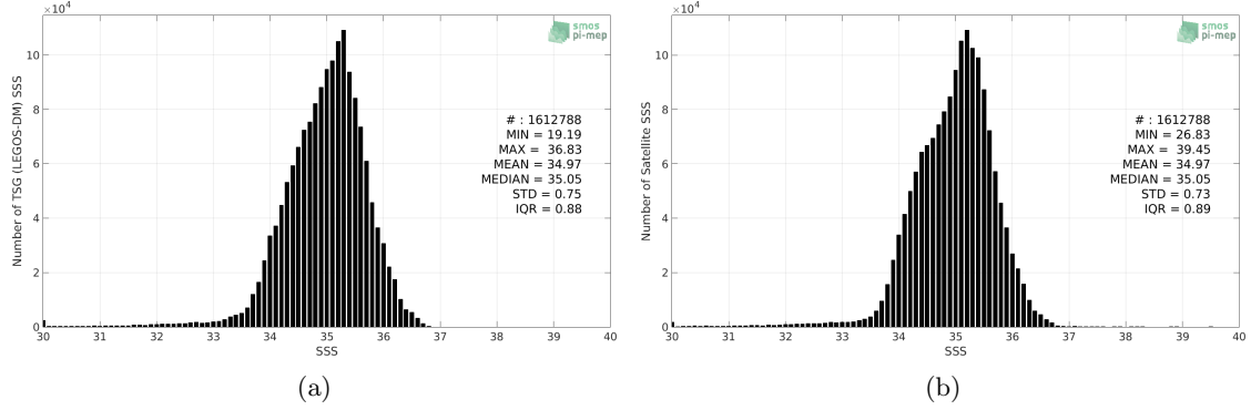
Figure 2: Histograms of SSS from TSG (LEGOS-DM) (a) and SMOS SSS L3 v5 - 18 Days (CATDS-CECOS-LOCEAN) (b) considering all match-up pairs per bins of 0.1 over the Tropical Pacific Ocean Pi-MEP region and for the full satellite product period.
