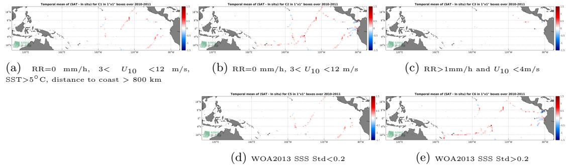
Figure 12: Temporal mean gridded over spatial boxes of size 1^\circ \times 1^\circ of \Delta SSS (SMOS SSS L3 v5 - 18 Days (CATDS-CECOS-LOCEAN) - TSG (GOSUD-Sailing-ship)) for 5 different subdatasets corresponding to: RR=0 mm/h, 3 < U_{10} < 12 m/s, SST > 5^\circ\text{C} , distance to coast > 800 km (a), RR=0 mm/h, 3 < U_{10} < 12 m/s (b), RR > 1\text{mm/h} and U_{10} < 4\text{m/s} (c), WOA2013 SSS Std < 0.2 (d), WOA2013 SSS Std > 0.2 (e).
