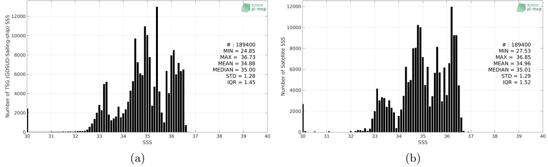
Figure 2: Histograms of SSS from TSG (GOSUD-Sailing-ship) (a) and SMOS SSS L3 v5 - 18 Days (CATDS-CECOS-LOCEAN) (b) considering all match-up pairs per bins of 0.1 over the Tropical Pacific Ocean Pi-MEP region and for the full satellite product period.
