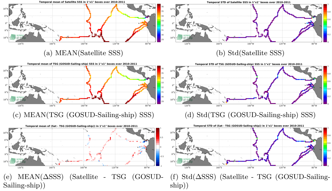
Figure 6: Temporal mean (left) and Std (right) of SSS from SMOS SSS L3 v5 - 18 Days (CATDS-CECOS-LOCEAN) (top), TSG (GOSUD-Sailing-ship) (middle), and of \Delta SSS (Satellite - TSG (GOSUD-Sailing-ship)). Only match-up pairs are used to generate these maps.
