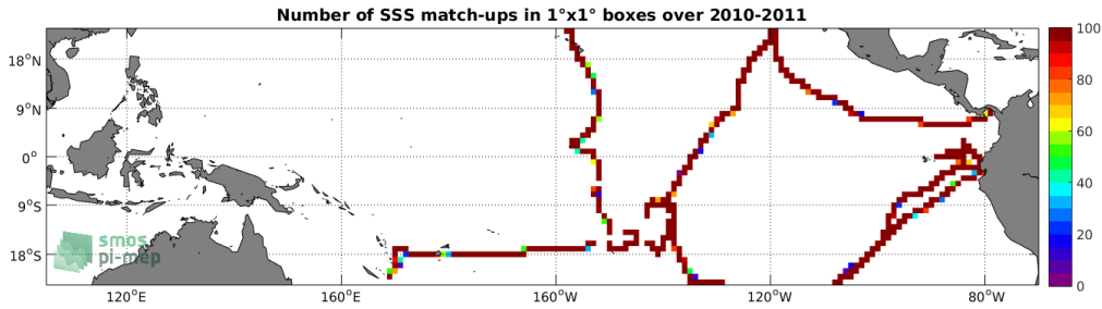
Figure 4: Number of SSS match-ups between TSG (GOSUD-Sailing-ship) SSS and the SMOS SSS L3 v5 - 18 Days (CATDS-CECOS-LOCEAN) SSS product for the Tropical Pacific Ocean Pi-MEP region over 1^\circ \times 1^\circ boxes and for the full satellite product period.
