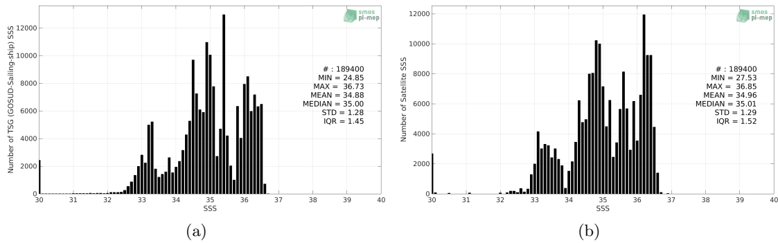
Figure 2: Histograms of SSS from TSG (GOSUD-Sailing-ship) (a) and SMOS SSS L3 v5 - 18 Days (CATDS-CECOS-LOCEAN) (b) considering all match-up pairs per bins of 0.1 over the Tropical Pacific Ocean Pi-MEP region and for the full satellite product period.
