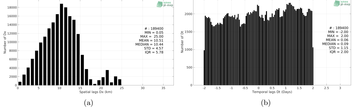
Figure 5: Histograms of the spatial (a) and temporal (b) lags between the time of the TSG (GOSUD-Sailing-ship) measurements and the date of the corresponding SMOS SSS L3 v5 - 18 Days (CATDS-CECOS-LOCEAN) SSS product.
