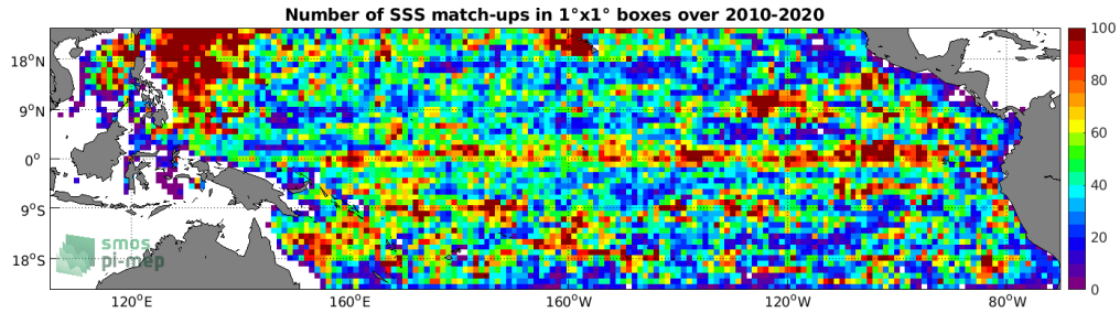
Figure 4: Number of SSS match-ups between Argo SSS and the SMOS SSS L3 v5 - 18 Days (CATDS-CECOS-LOCEAN) SSS product for the Tropical Pacific Ocean Pi-MEP region over 1^\circ \times 1^\circ boxes and for the full satellite product period.
