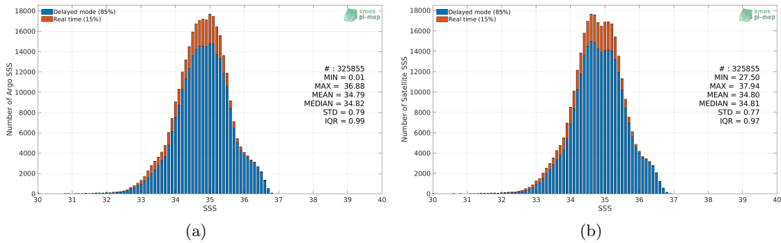
Figure 2: Histograms of SSS from Argo (a) and SMOS SSS L3 v5 - 18 Days (CATDS-CECOS-LOCEAN) (b) considering all match-up pairs per bins of 0.1 over the Tropical Pacific Ocean Pi-MEP region and for the full satellite product period.
