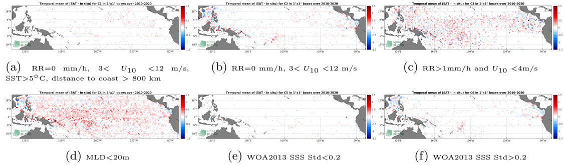
Figure 12: Temporal mean gridded over spatial boxes of size 1^\circ \times 1^\circ of \Delta SSS (SMOS SSS L3 v5 - 18 Days (CATDS-CECOS-LOCEAN) - Argo) for 6 different subdatasets corresponding to: RR=0 mm/h, 3 < U_{10} < 12 m/s, SST > 5^\circ\text{C} , distance to coast > 800 km (a), RR=0 mm/h, 3 < U_{10} < 12 m/s (b), RR > 1 mm/h and U_{10} < 4 m/s (c), MLD < 20 m (d), WOA2013 SSS Std < 0.2 (e), WOA2013 SSS Std > 0.2 (f).
