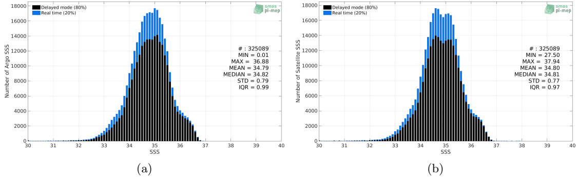
Figure 2: Histograms of SSS from Argo (a) and SMOS SSS L3 v5 - 18 Days (CATDS-CECOS-LOCEAN) (b) considering all match-up pairs per bins of 0.1 over the Tropical Pacific Ocean Pi-MEP region and for the full satellite product period.
