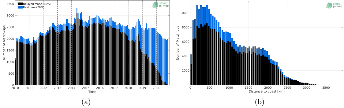
Figure 1: Number of match-ups between Argo and SMOS SSS L3 v5 - 18 Days (CATDS-CECOS-LOCEAN) SSS as a function of time (a) and as function of the distance to coast (b) over the Tropical Pacific Ocean Pi-MEP region and for the full satellite product period.
