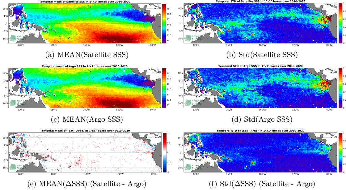
Figure 6: Temporal mean (left) and Std (right) of SSS from SMOS SSS L3 v5 - 18 Days (CATDS-CECOS-LOCEAN) (top), Argo (middle), and of \Delta SSS (Satellite - Argo). Only match-up pairs are used to generate these maps.
