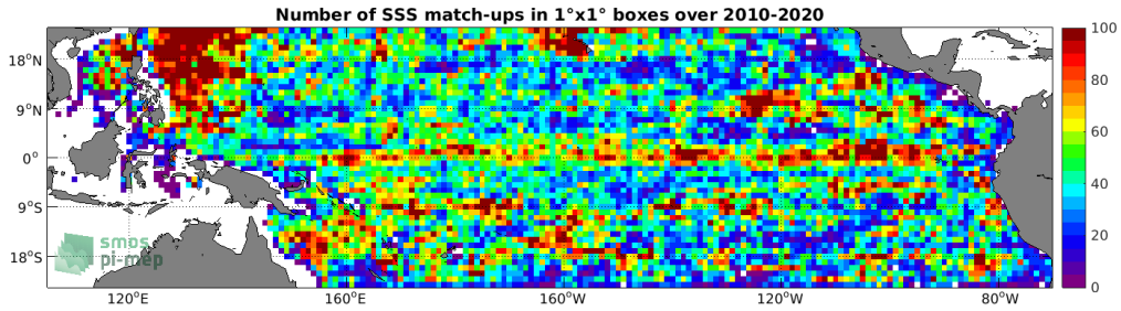
Figure 4: Number of SSS match-ups between Argo SSS and the SMOS SSS L3 v5 - 18 Days (CATDS-CECOS-LOCEAN) SSS product for the Tropical Pacific Ocean Pi-MEP region over 1^\circ \times 1^\circ boxes and for the full satellite product period.
