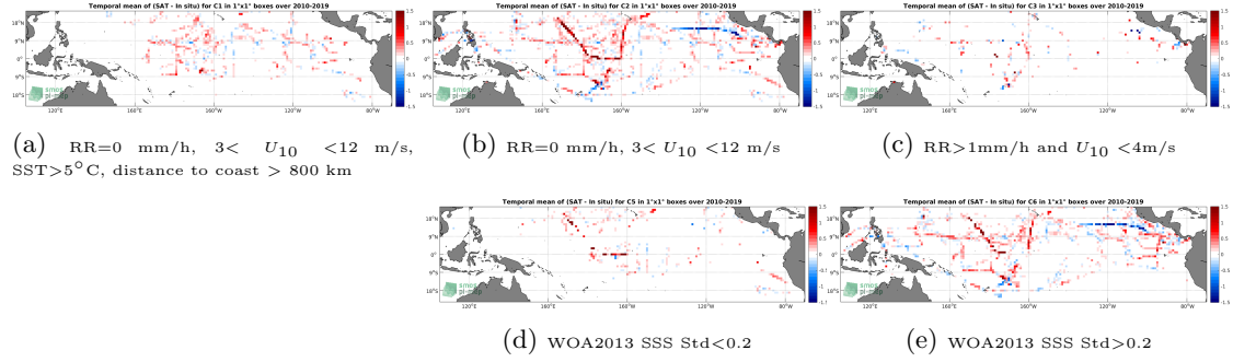
Figure 12: Temporal mean gridded over spatial boxes of size 1^{\circ}\times 1^{\circ} of \Delta\text{SSS} (SMOS SSS L3 v4 - 9 Days (CATDS-CECOS-LOCEAN) - TSG (SAMOS)) for 5 different subdatasets corresponding to: \text{RR}=0 mm/h, 3 < U_{10} < 12 m/s, \text{SST}>5^{\circ}\text{C} , distance to coast > 800 km (a), \text{RR}=0 mm/h, 3 < U_{10} < 12 m/s (b), \text{RR}>1\text{mm/h} and U_{10} < 4\text{m/s} (c), WOA2013 SSS Std <0.2 (d), WOA2013 SSS Std >0.2 (e).
