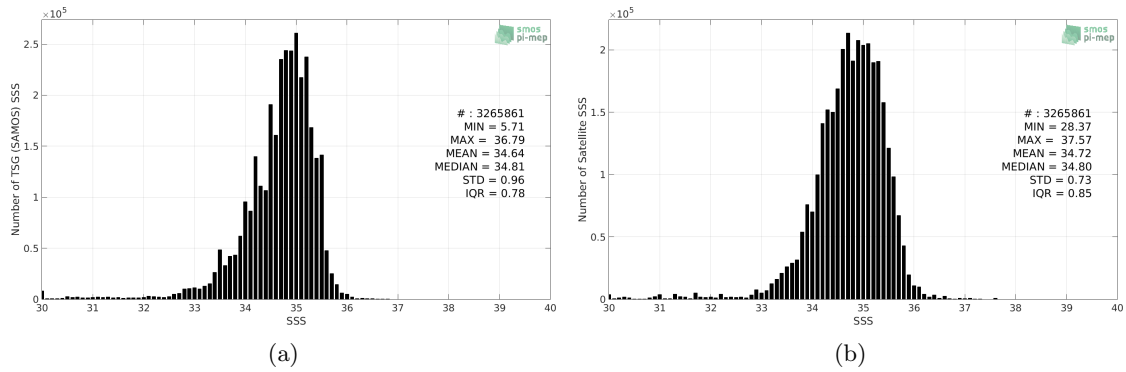
Figure 2: Histograms of SSS from TSG (SAMOS) (a) and SMOS SSS L3 v4 - 9 Days (CATDS-CECOS-LOCEAN) (b) considering all match-up pairs per bins of 0.1 over the Tropical Pacific Ocean Pi-MEP region and for the full satellite product period.
