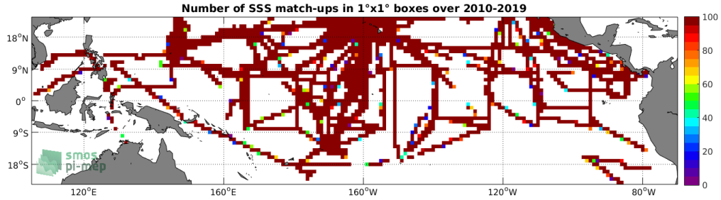
Figure 4: Number of SSS match-ups between TSG (SAMOS) SSS and the SMOS SSS L3 v4 - 9 Days (CATDS-CECOS-LOCEAN) SSS product for the Tropical Pacific Ocean Pi-MEP region over 1^\circ \times 1^\circ boxes and for the full satellite product period.
