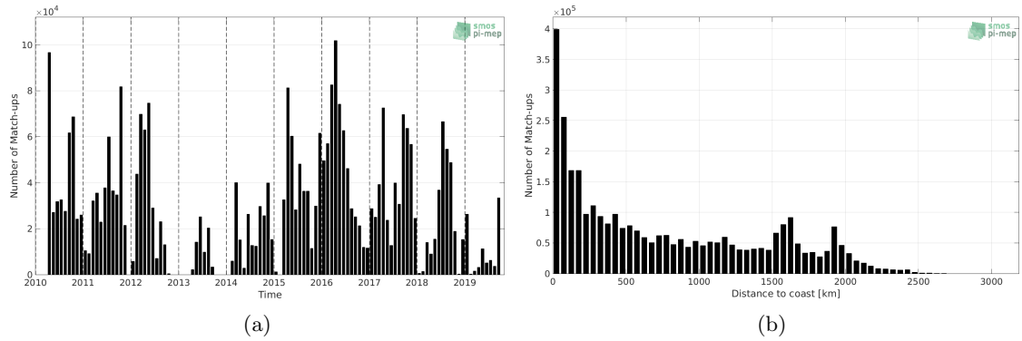
Figure 1: Number of match-ups between TSG (SAMOS) and SMOS SSS L3 v4 - 9 Days (CATDS-CECOS-LOCEAN) SSS as a function of time (a) and as function of the distance to coast (b) over the Tropical Pacific Ocean Pi-MEP region and for the full satellite product period.
