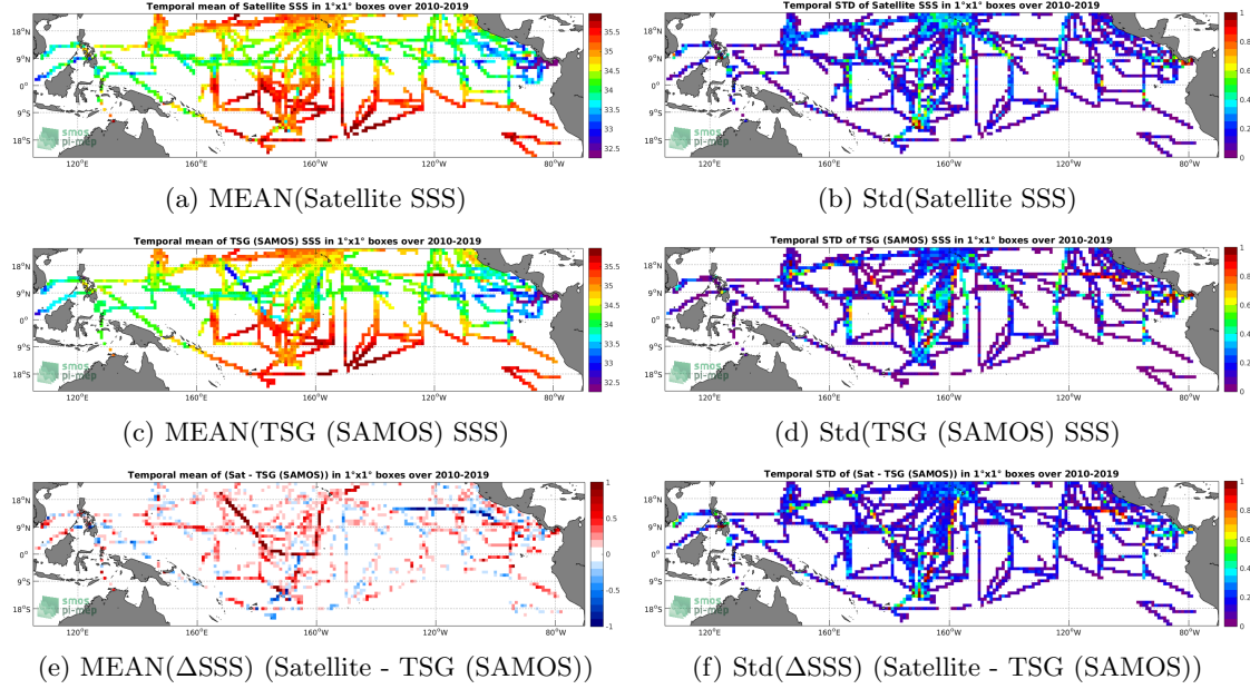
Figure 6: Temporal mean (left) and Std (right) of SSS from SMOS SSS L3 v4 - 9 Days (CATDS-CECOS-LOCEAN) (top), TSG (SAMOS) (middle), and of \Delta SSS (Satellite - TSG (SAMOS)). Only match-up pairs are used to generate these maps.
