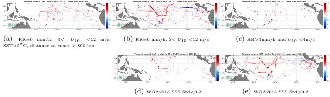
Figure 12: Temporal mean gridded over spatial boxes of size 1^{\circ}\times 1^{\circ} of \Delta\text{SSS} (SMOS-L3-CATDS-CECOS-LOCEAN-V4-9DAYS-25KM - TSG-SAMOS) for 5 different subdatasets corresponding to:RR=0 mm/h, 3 < U_{10} < 12 m/s, SST >5^{\circ}\text{C} , distance to coast > 800 km (a), RR=0 mm/h, 3 < U_{10} < 12 m/s (b), RR >1 mm/h and U_{10} < 4 m/s (c), WOA2013 SSS Std <0.2 (d), WOA2013 SSS Std >0.2 (e).
