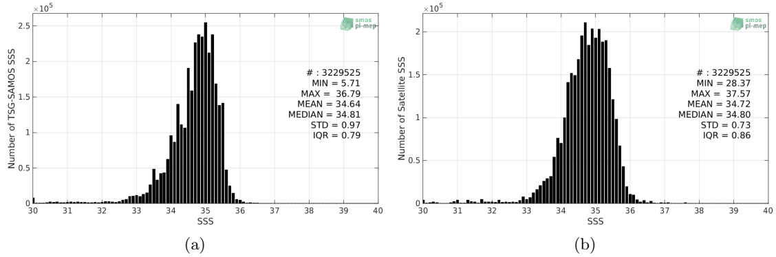
Figure 2: Histograms of SSS from TSG-SAMOS (a) and SMOS-L3-CATDS-CECOS-LOCEAN-V4-9DAYS-25KM (b) considering all match-up pairs per bins of 0.1 over the Tropical Pacific Ocean Pi-MEP region and for the full satellite product period.
