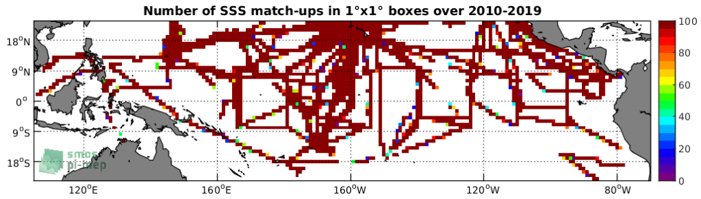
Figure 4: Number of SSS match-ups between TSG-SAMOS SSS and the SMOS-L3-CATDS-CECOS-LOCEAN-V4-9DAYS-25KM SSS product for the Tropical Pacific Ocean Pi-MEP region over 1^\circ \times 1^\circ boxes and for the full satellite product period.
