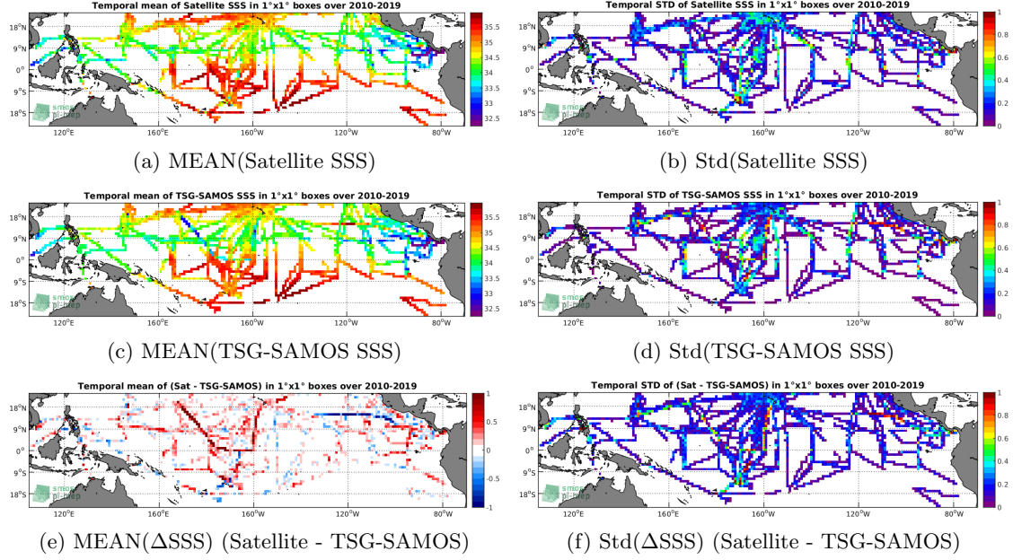
Figure 6: Temporal mean (left) and Std (right) of SSS from SMOS-L3-CATDS-CECOS-LOCEAN-V4-9DAYS-25KM (top), TSG-SAMOS (middle), and of \Delta SSS (Satellite - TSG-SAMOS). Only match-up pairs are used to generate these maps.
