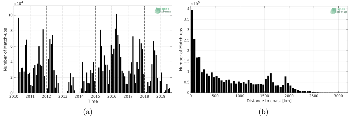
Figure 1: Number of match-ups between TSG-SAMOS and SMOS-L3-CATDS-CECOS-LOCEAN-V4-9DAYS-25KM SSS as a function of time (a) and as function of the distance to coast (b) over the Tropical Pacific Ocean Pi-MEP region and for the full satellite product period.
