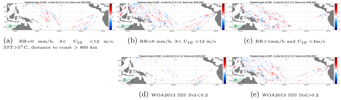
Figure 12: Temporal mean gridded over spatial boxes of size 1^{\circ}\times 1^{\circ} of \Delta\text{SSS} (SMOS-L3-CATDS-CECOS-LOCEAN-V4-9DAYS-25KM - TSG-LEGOS-DM) for 5 different subdatasets corresponding to:RR=0 mm/h, 3 < U_{10} < 12 m/s, SST >5^{\circ}\text{C} , distance to coast > 800 km (a), RR=0 mm/h, 3 < U_{10} < 12 m/s (b), RR >1 mm/h and U_{10} < 4 m/s (c), WOA2013 SSS Std <0.2 (d), WOA2013 SSS Std >0.2 (e).
