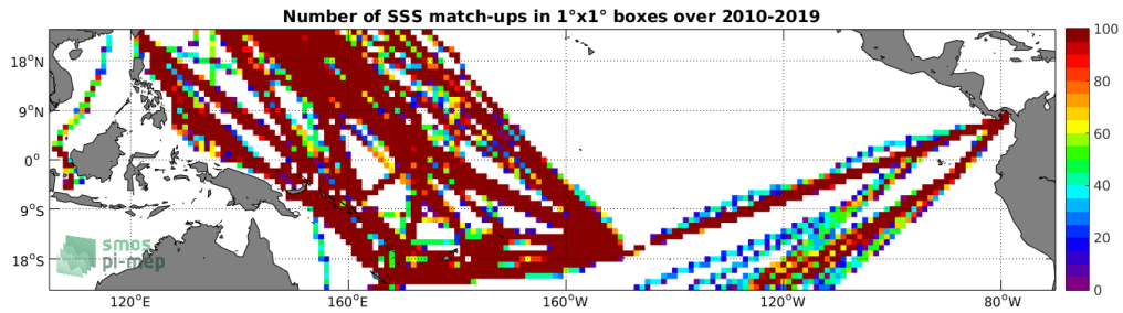
Figure 4: Number of SSS match-ups between TSG-LEGOS-DM SSS and the SMOS-L3-CATDS-CECOS-LOCEAN-V4-9DAYS-25KM SSS product for the Tropical Pacific Ocean Pi-MEP region over 1^\circ \times 1^\circ boxes and for the full satellite product period.
