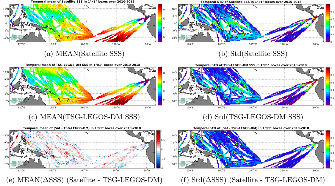
Figure 6: Temporal mean (left) and Std (right) of SSS from SMOS-L3-CATDS-CECOS-LOCEAN-V4-9DAYS-25KM (top), TSG-LEGOS-DM (middle), and of \Delta SSS (Satellite - TSG-LEGOS-DM). Only match-up pairs are used to generate these maps.
