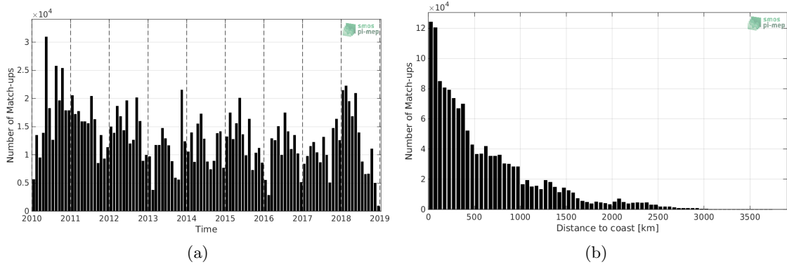
Figure 1: Number of match-ups between TSG-LEGOS-DM and SMOS-L3-CATDS-CECOS-LOCEAN-V4-9DAYS-25KM SSS as a function of time (a) and as function of the distance to coast (b) over the Tropical Pacific Ocean Pi-MEP region and for the full satellite product period.
