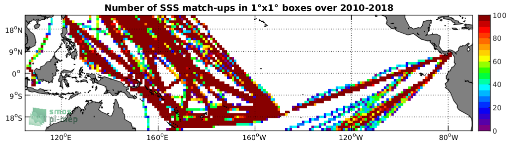
Figure 4: Number of SSS match-ups between TSG-LEGOS-DM SSS and the SMOS-L3-CATDS-CECOS-LOCEAN-V4-9DAYS-25KM SSS product for the Tropical Pacific Ocean Pi-MEP region over 1°x1° boxes and for the full satellite product period.
