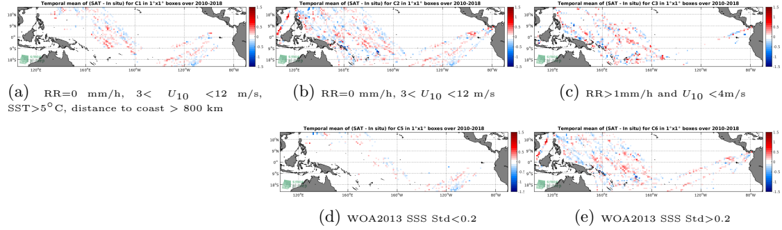
Figure 12: Temporal mean gridded over spatial boxes of size 1^\circ \times 1^\circ of \Delta SSS (SMOS-L3-CATDS-CECOS-LOCEAN-V4-9DAYS-25KM - TSG-LEGOS-DM) for 5 different subdatasets corresponding to: RR=0 mm/h, 3 < U_{10} < 12 m/s, SST > 5^\circ\text{C} , distance to coast > 800 km (a), RR=0 mm/h, 3 < U_{10} < 12 m/s (b), RR > 1 mm/h and U_{10} < 4 m/s (c), WOA2013 SSS Std < 0.2 (d), WOA2013 SSS Std > 0.2 (e).
