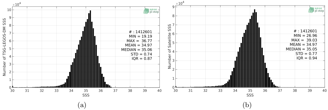
Figure 2: Histograms of SSS from TSG-LEGOS-DM (a) and SMOS-L3-CATDS-CECOS-LOCEAN-V4-9DAYS-25KM (b) considering all match-up pairs per bins of 0.1 over the Tropical Pacific Ocean Pi-MEP region and for the full satellite product period.
