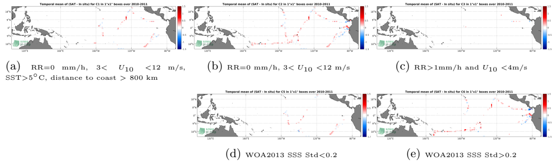
Figure 12: Temporal mean gridded over spatial boxes of size 1^\circ \times 1^\circ of \Delta SSS (SMOS SSS L3 v4 - 9 Days (CATDS-CECOS-LOCEAN) - TSG (GOSUD-Sailing-ship)) for 5 different subdatasets corresponding to: RR=0 mm/h, 3 < U_{10} < 12 m/s, SST > 5^\circ\text{C} , distance to coast > 800 km (a), RR=0 mm/h, 3 < U_{10} < 12 m/s (b), RR > 1\text{mm/h} and U_{10} < 4\text{m/s} (c), WOA2013 SSS Std < 0.2 (d), WOA2013 SSS Std > 0.2 (e).
