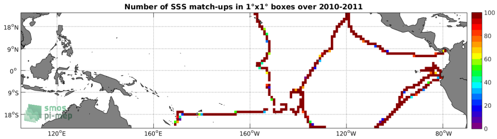
Figure 4: Number of SSS match-ups between TSG (GOSUD-Sailing-ship) SSS and the SMOS SSS L3 v4 - 9 Days (CATDS-CECOS-LOCEAN) SSS product for the Tropical Pacific Ocean Pi-MEP region over 1^\circ \times 1^\circ boxes and for the full satellite product period.
