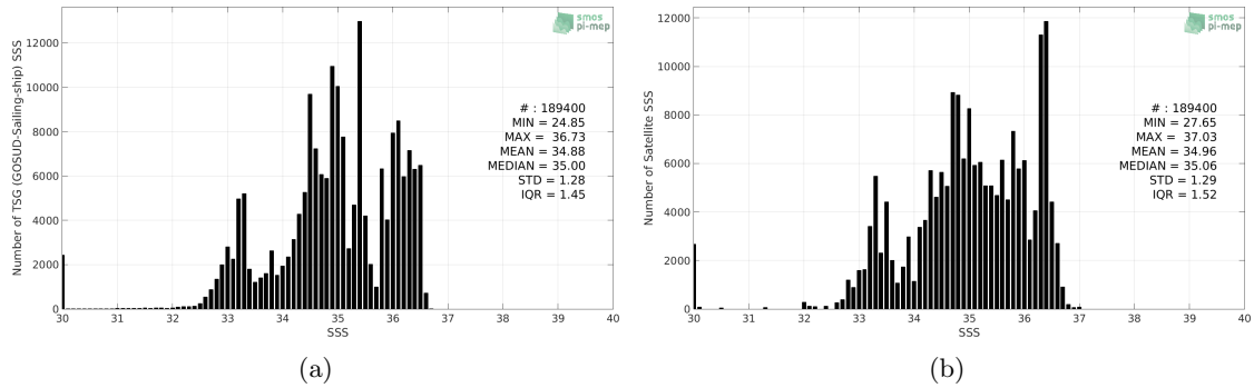
Figure 2: Histograms of SSS from TSG (GOSUD-Sailing-ship) (a) and SMOS SSS L3 v4 - 9 Days (CATDS-CECOS-LOCEAN) (b) considering all match-up pairs per bins of 0.1 over the Tropical Pacific Ocean Pi-MEP region and for the full satellite product period.
