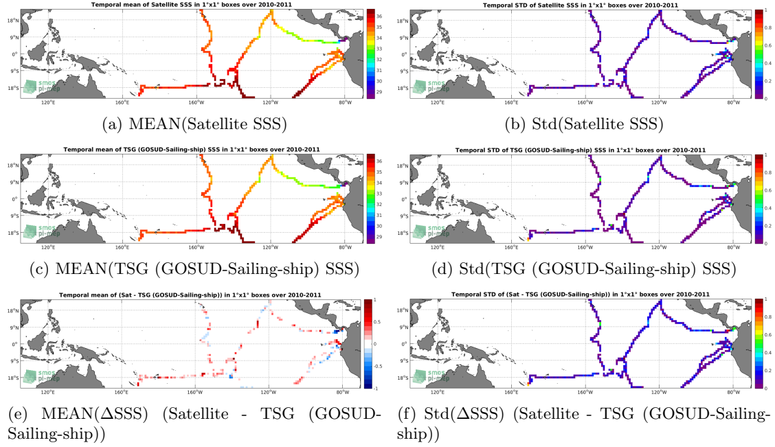
Figure 6: Temporal mean (left) and Std (right) of SSS from SMOS SSS L3 v4 - 9 Days (CATDS-CECOS-LOCEAN) (top), TSG (GOSUD-Sailing-ship) (middle), and of \Delta SSS (Satellite - TSG (GOSUD-Sailing-ship)). Only match-up pairs are used to generate these maps.
