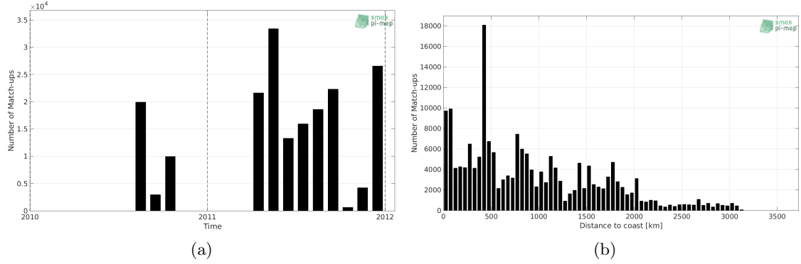
Figure 1: Number of match-ups between TSG (GOSUD-Sailing-ship) and SMOS SSS L3 v4 - 9 Days (CATDS-CECOS-LOCEAN) SSS as a function of time (a) and as function of the distance to coast (b) over the Tropical Pacific Ocean Pi-MEP region and for the full satellite product period.
