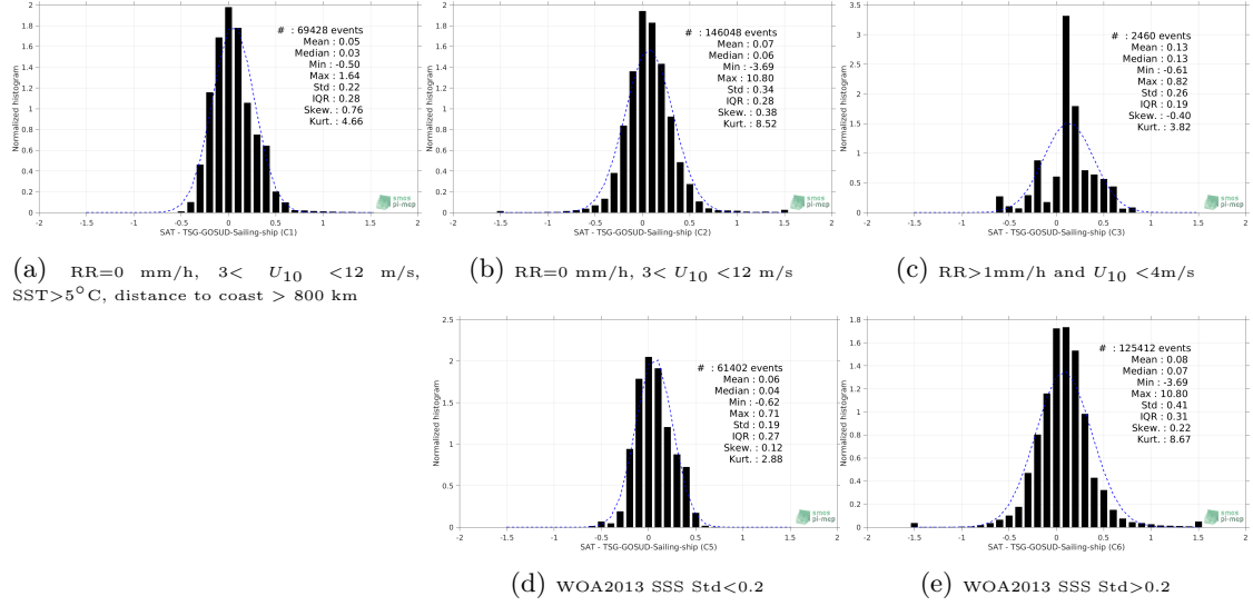
Figure 13: Normalized histogram of \Delta SSS (SMOS-L3-CATDS-CECOS-LOCEAN-V4-9DAYS-25KM - TSG-GOSUD-Sailing-ship) for 5 different subdatasets corresponding to: RR=0 mm/h, 3 < U_{10} < 12 m/s, SST > 5^\circ\text{C} , distance to coast > 800 km (a), RR=0 mm/h, 3 < U_{10} < 12 m/s (b), RR > 1 mm/h and U_{10} < 4 m/s (c), WOA2013 SSS Std < 0.2 (d), WOA2013 SSS Std > 0.2 (e).
