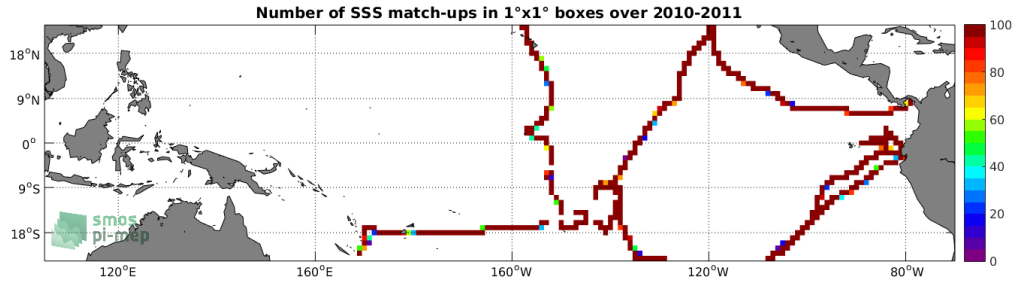
Figure 4: Number of SSS match-ups between TSG-GOSUD-Sailing-ship SSS and the SMOS-L3-CATDS-CECOS-LOCEAN-V4-9DAYS-25KM SSS product for the Tropical Pacific Ocean Pi-MEP region over 1^\circ \times 1^\circ boxes and for the full satellite product period.
