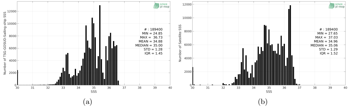
Figure 2: Histograms of SSS from TSG-GOSUD-Sailing-ship (a) and SMOS-L3-CATDS-CECOS-LOCEAN-V4-9DAYS-25KM (b) considering all match-up pairs per bins of 0.1 over the Tropical Pacific Ocean Pi-MEP region and for the full satellite product period.
