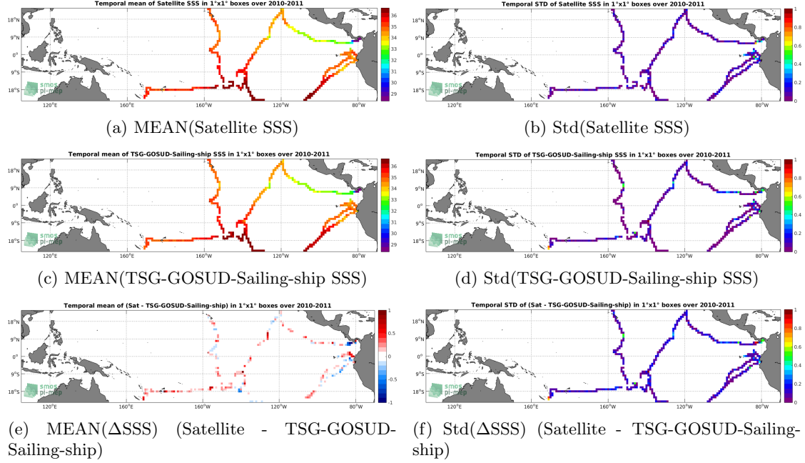
Figure 6: Temporal mean (left) and Std (right) of SSS from SMOS-L3-CATDS-CECOS-LOCEAN-V4-9DAYS-25KM (top), TSG-GOSUD-Sailing-ship (middle), and of \Delta SSS (Satellite - TSG-GOSUD-Sailing-ship). Only match-up pairs are used to generate these maps.
