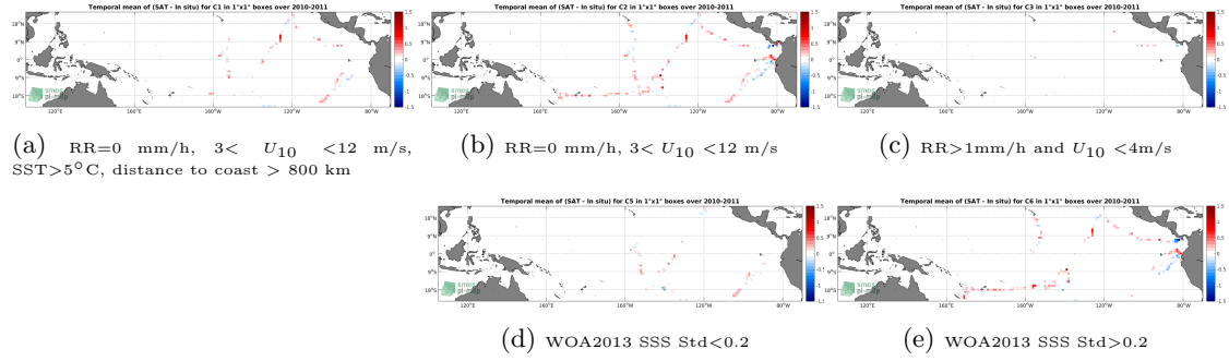
Figure 12: Temporal mean gridded over spatial boxes of size 1^\circ \times 1^\circ of \Delta SSS (SMOS-L3-CATDS-CECOS-LOCEAN-V4-9DAYS-25KM - TSG-GOSUD-Sailing-ship) for 5 different subdatasets corresponding to: RR=0 mm/h, 3 < U_{10} < 12 m/s, SST >5^\circ\text{C} , distance to coast > 800 km (a), RR=0 mm/h, 3 < U_{10} < 12 m/s (b), RR >1 mm/h and U_{10} < 4 m/s (c), WOA2013 SSS Std <0.2 (d), WOA2013 SSS Std >0.2 (e).
