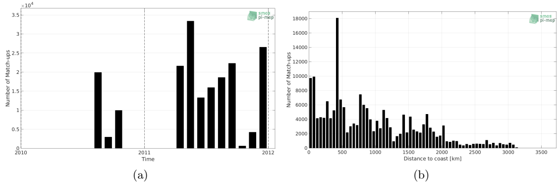
Figure 1: Number of match-ups between TSG-GOSUD-Sailing-ship and SMOS-L3-CATDS-CECOS-LOCEAN-V4-9DAYS-25KM SSS as a function of time (a) and as function of the distance to coast (b) over the Tropical Pacific Ocean Pi-MEP region and for the full satellite product period.
