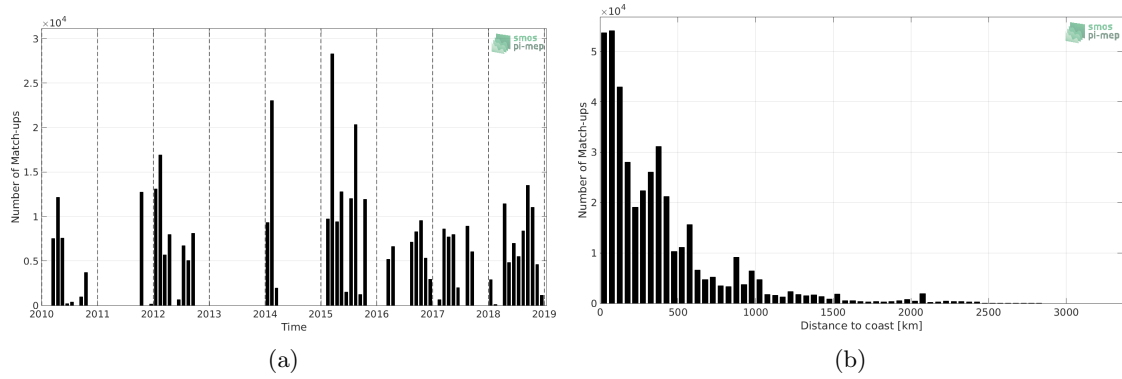
Figure 1: Number of match-ups between TSG (GOSUD-Research-vessel) and SMOS SSS L3 v4 - 9 Days (CATDS-CECOS-LOCEAN) SSS as a function of time (a) and as function of the distance to coast (b) over the Tropical Pacific Ocean Pi-MEP region and for the full satellite product period.
