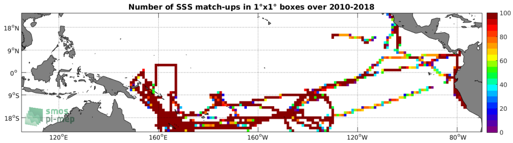
Figure 4: Number of SSS match-ups between TSG (GOSUD-Research-vessel) SSS and the SMOS SSS L3 v4 - 9 Days (CATDS-CECOS-LOCEAN) SSS product for the Tropical Pacific Ocean Pi-MEP region over 1^\circ \times 1^\circ boxes and for the full satellite product period.
