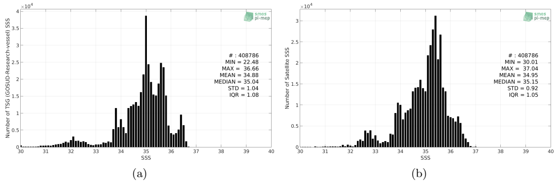
Figure 2: Histograms of SSS from TSG (GOSUD-Research-vessel) (a) and SMOS SSS L3 v4 - 9 Days (CATDS-CECOS-LOCEAN) (b) considering all match-up pairs per bins of 0.1 over the Tropical Pacific Ocean Pi-MEP region and for the full satellite product period.
