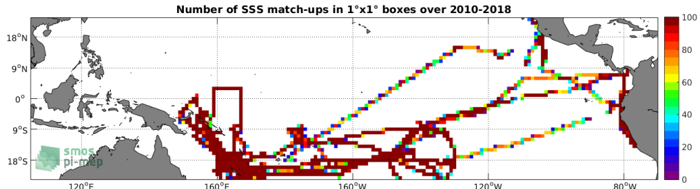
Figure 4: Number of SSS match-ups between TSG-GOSUD-Research-vessel SSS and the SMOS-L3-CATDS-CECOS-LOCEAN-V4-9DAYS-25KM SSS product for the Tropical Pacific Ocean Pi-MEP region over 1°x1° boxes and for the full satellite product period.
