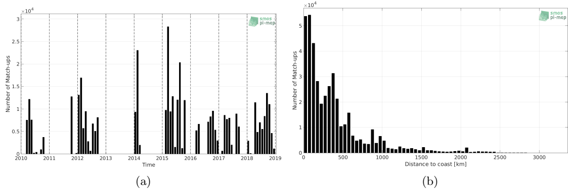
Figure 1: Number of match-ups between TSG-GOSUD-Research-vessel and SMOS-L3-CATDS-CECOS-LOCEAN-V4-9DAYS-25KM SSS as a function of time (a) and as function of the distance to coast (b) over the Tropical Pacific Ocean Pi-MEP region and for the full satellite product period.
