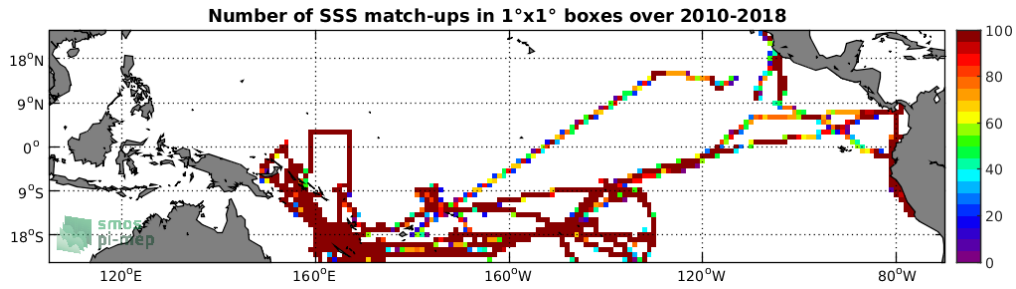
Figure 4: Number of SSS match-ups between TSG-GOSUD-Research-vessel SSS and the SMOS-L3-CATDS-CECOS-LOCEAN-V4-9DAYS-25KM SSS product for the Tropical Pacific Ocean Pi-MEP region over 1^\circ \times 1^\circ boxes and for the full satellite product period.
