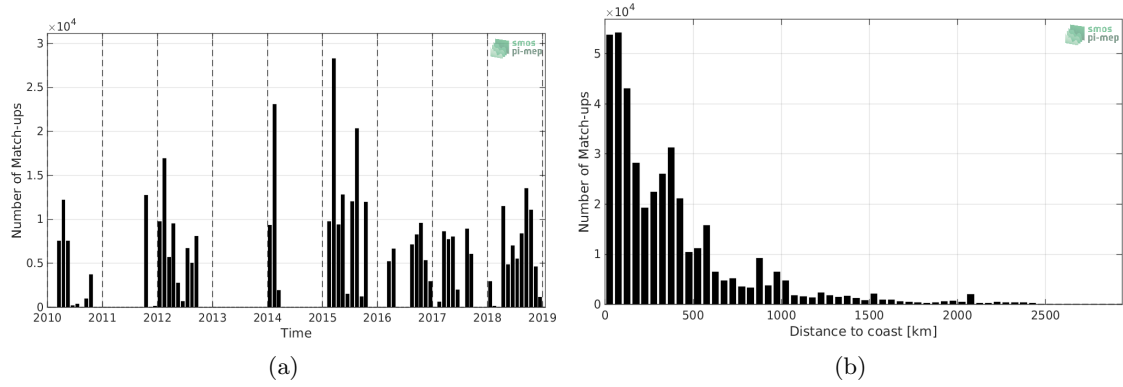
Figure 1: Number of match-ups between TSG-GOSUD-Research-vessel and SMOS-L3-CATDS-CECOS-LOCEAN-V4-9DAYS-25KM SSS as a function of time (a) and as function of the distance to coast (b) over the Tropical Pacific Ocean Pi-MEP region and for the full satellite product period.
