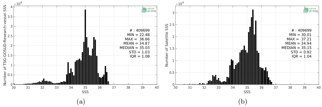
Figure 2: Histograms of SSS from TSG-GOSUD-Research-vessel (a) and SMOS-L3-CATDS-CECOS-LOCEAN-V4-9DAYS-25KM (b) considering all match-up pairs per bins of 0.1 over the Tropical Pacific Ocean Pi-MEP region and for the full satellite product period.
