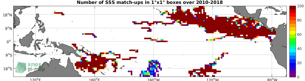
Figure 3: Number of SSS match-ups between Surface drifters SSS and the SMOS SSS L3 v4 - 9 Days (CATDS-CECOS-LOCEAN) SSS product for the Tropical Pacific Ocean Pi-MEP region over 1^\circ \times 1^\circ boxes and for the full satellite product period.
