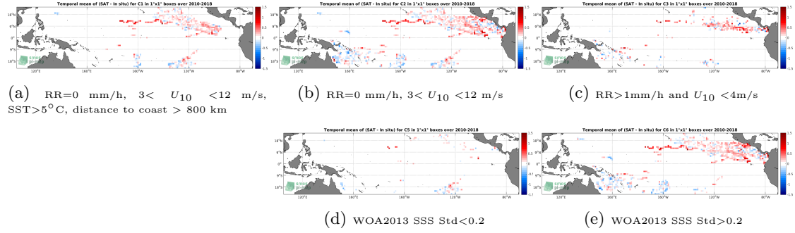
Figure 11: Temporal mean gridded over spatial boxes of size 1^{\circ}\times 1^{\circ} of \Delta\text{SSS} (SMOS SSS L3 v4 - 9 Days (CATDS-CECOS-LOCEAN) - Surface drifters) for 5 different subdatasets corresponding to:RR=0 mm/h, 3 < U_{10} < 12 m/s, SST >5^{\circ}\text{C} , distance to coast > 800 km (a), RR=0 mm/h, 3 < U_{10} < 12 m/s (b), RR >1 mm/h and U_{10} < 4 m/s (c), WOA2013 SSS Std <0.2 (d), WOA2013 SSS Std >0.2 (e).
