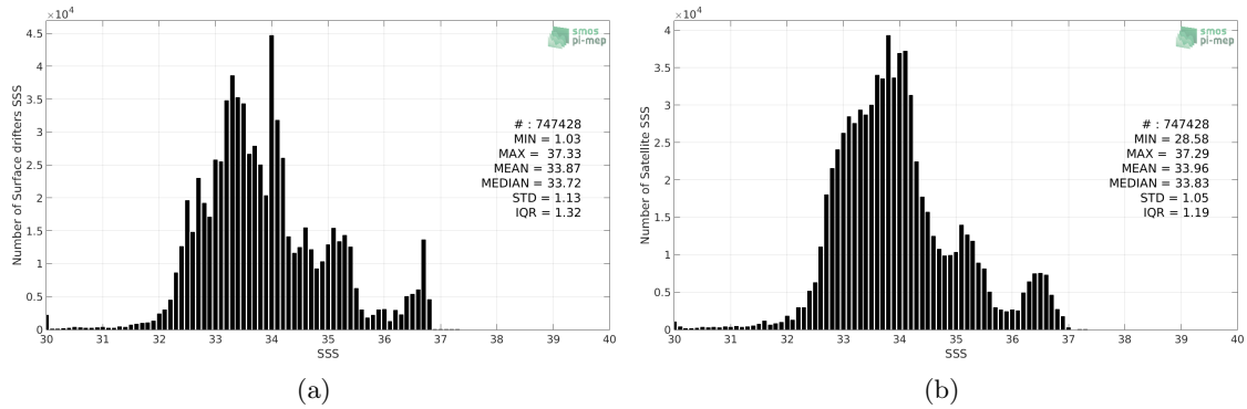
Figure 2: Histograms of SSS from Surface drifters (a) and SMOS SSS L3 v4 - 9 Days (CATDS-CECOS-LOCEAN) (b) considering all match-up pairs per bins of 0.1 over the Tropical Pacific Ocean Pi-MEP region and for the full satellite product period.
