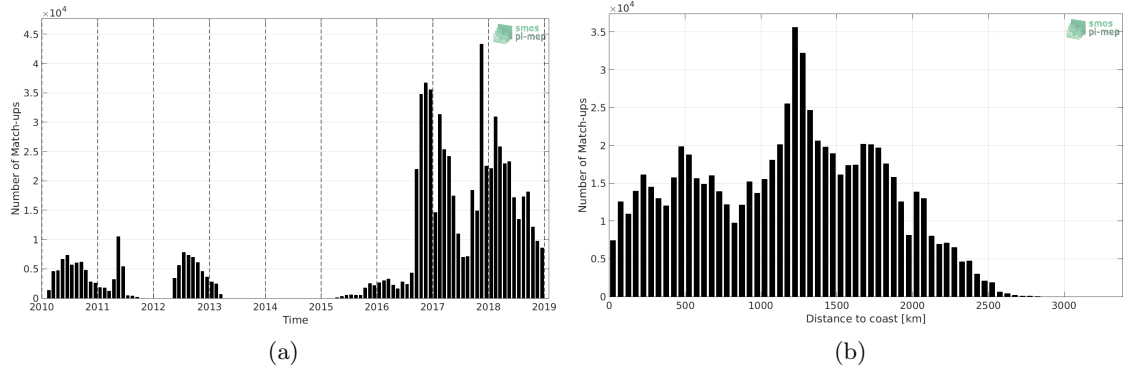
Figure 1: Number of match-ups between Surface drifters and SMOS SSS L3 v4 - 9 Days (CATDS-CECOS-LOCEAN) SSS as a function of time (a) and as function of the distance to coast (b) over the Tropical Pacific Ocean Pi-MEP region and for the full satellite product period.
