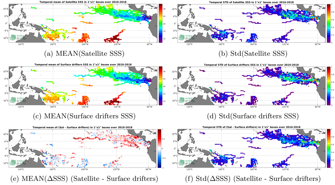
Figure 5: Temporal mean (left) and Std (right) of SSS from SMOS SSS L3 v4 - 9 Days (CATDS-CECOS-LOCEAN) (top), Surface drifters (middle), and of \Delta SSS (Satellite - Surface drifters). Only match-up pairs are used to generate these maps.
