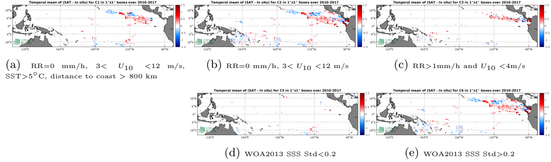
Figure 11: Temporal mean gridded over spatial boxes of size 1^\circ \times 1^\circ of \Delta SSS (SMOS-L3-CATDS-CECOS-LOCEAN-V4-9DAYS-25KM - Surface drifters) for 5 different subdatasets corresponding to: RR=0 mm/h, 3 < U_{10} < 12 m/s, SST > 5^\circ C , distance to coast > 800 km (a), RR=0 mm/h, 3 < U_{10} < 12 m/s (b), RR > 1 mm/h and U_{10} < 4 m/s (c), WOA2013 SSS Std < 0.2 (d), WOA2013 SSS Std > 0.2 (e).
