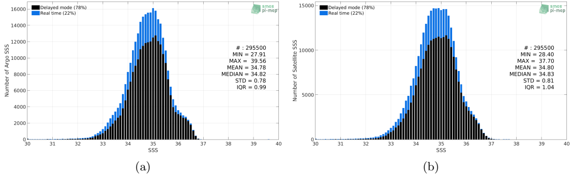
Figure 2: Histograms of SSS from Argo (a) and SMOS-L3-CATDS-CECOS-LOCEAN-V4-9DAYS-25KM (b) considering all match-up pairs per bins of 0.1 over the Tropical Pacific Ocean Pi-MEP region and for the full satellite product period.
