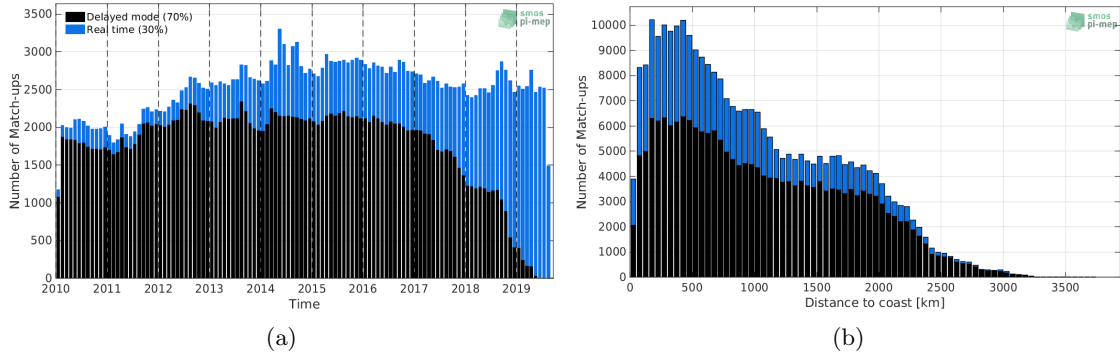
Figure 1: Number of match-ups between Argo and SMOS-L3-CATDS-CECOS-LOCEAN-V4-9DAYS-25KM SSS as a function of time (a) and as function of the distance to coast (b) over the Tropical Pacific Ocean Pi-MEP region and for the full satellite product period.
