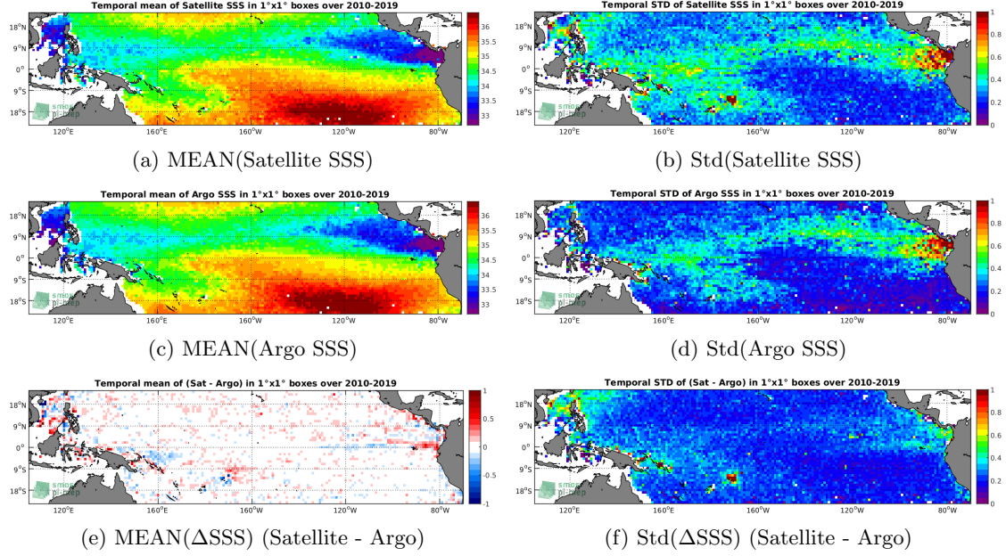
Figure 6: Temporal mean (left) and Std (right) of SSS from SMOS-L3-CATDS-CECOS-LOCEAN-V4-9DAYS-25KM (top), Argo (middle), and of \Delta SSS (Satellite - Argo). Only match-up pairs are used to generate these maps.
