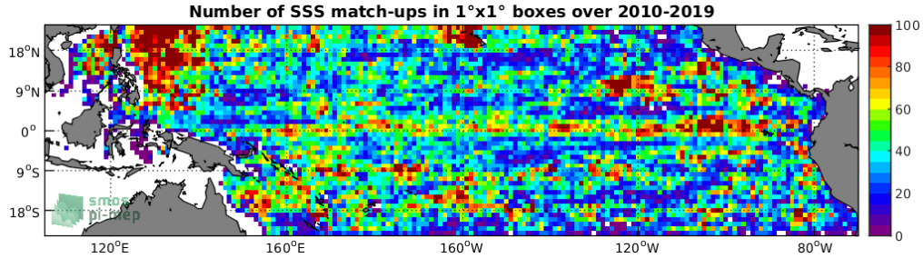
Figure 4: Number of SSS match-ups between Argo SSS and the SMOS-L3-CATDS-CECOS-LOCEAN-V4-9DAYS-25KM SSS product for the Tropical Pacific Ocean Pi-MEP region over 1^\circ \times 1^\circ boxes and for the full satellite product period.
