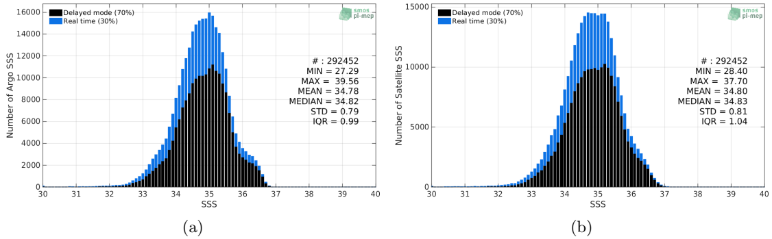
Figure 2: Histograms of SSS from Argo (a) and SMOS-L3-CATDS-CECOS-LOCEAN-V4-9DAYS-25KM (b) considering all match-up pairs per bins of 0.1 over the Tropical Pacific Ocean Pi-MEP region and for the full satellite product period.
