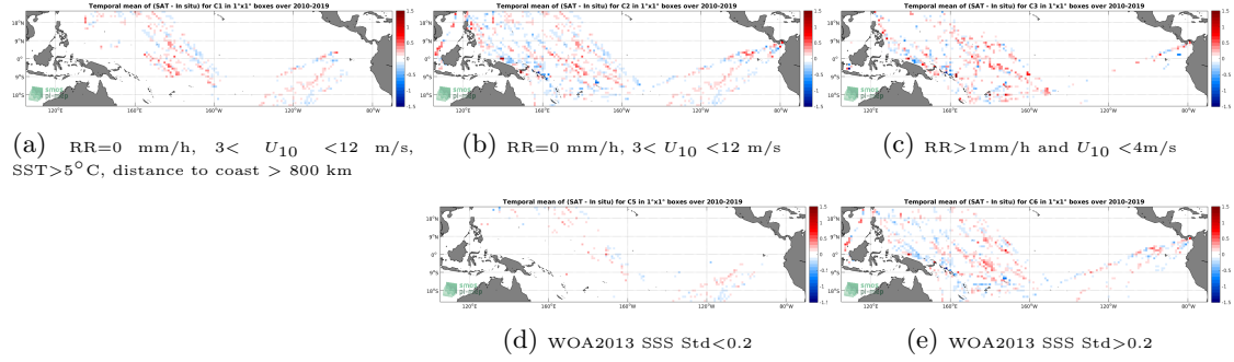
Figure 12: Temporal mean gridded over spatial boxes of size 1^{\circ}\times 1^{\circ} of \Delta\text{SSS} (SMOS SSS L3 v4 - 18 Days (CATDS-CECOS-LOCEAN) - TSG (LEGOS-DM)) for 5 different subdatasets corresponding to: \text{RR}=0 mm/h, 3 < U_{10} < 12 m/s, \text{SST} > 5^{\circ}\text{C} , distance to coast > 800 km (a), \text{RR}=0 mm/h, 3 < U_{10} < 12 m/s (b), \text{RR} > 1 mm/h and U_{10} < 4 m/s (c), WOA2013 SSS Std < 0.2 (d), WOA2013 SSS Std > 0.2 (e).
