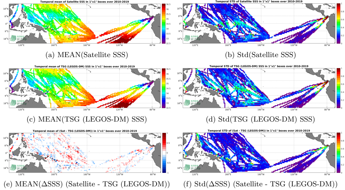
Figure 6: Temporal mean (left) and Std (right) of SSS from SMOS SSS L3 v4 - 18 Days (CATDS-CECOS-LOCEAN) (top), TSG (LEGOS-DM) (middle), and of \Delta SSS (Satellite - TSG (LEGOS-DM)). Only match-up pairs are used to generate these maps.
