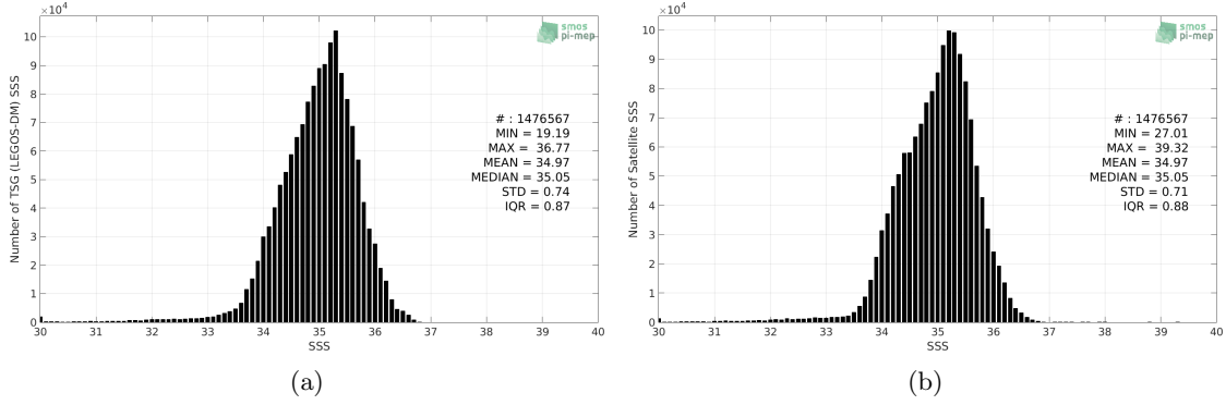
Figure 2: Histograms of SSS from TSG (LEGOS-DM) (a) and SMOS SSS L3 v4 - 18 Days (CATDS-CECOS-LOCEAN) (b) considering all match-up pairs per bins of 0.1 over the Tropical Pacific Ocean Pi-MEP region and for the full satellite product period.
