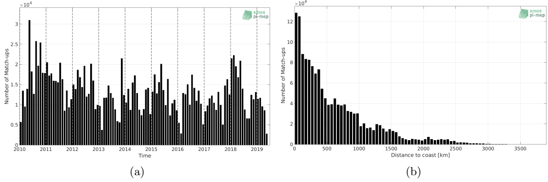
Figure 1: Number of match-ups between TSG (LEGOS-DM) and SMOS SSS L3 v4 - 18 Days (CATDS-CECOS-LOCEAN) SSS as a function of time (a) and as function of the distance to coast (b) over the Tropical Pacific Ocean Pi-MEP region and for the full satellite product period.
