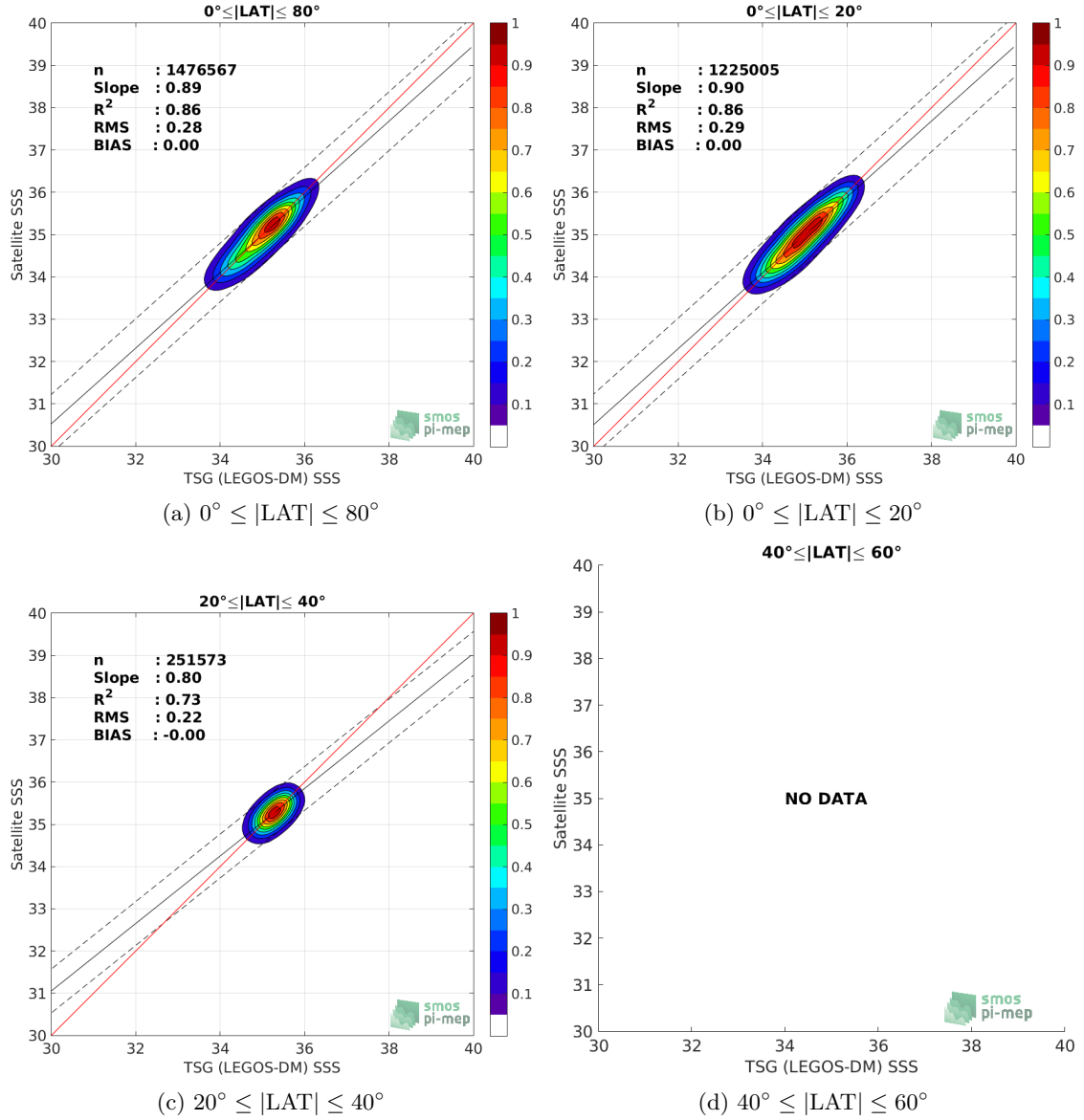
Figure 9: Contour maps of the concentration of SMOS SSS L3 v4 - 18 Days (CATDS-CECOS-LOCEAN) SSS (y-axis) versus TSG (LEGOS-DM) SSS (x-axis) at match-up pairs for different latitude bands. For each plot, the red line shows x=y . The black thin and dashed lines indicate a linear fit through the data cloud and the \pm 95\% confidence levels, respectively. The number match-up pairs n , the slope and R^2 coefficient of the linear fit, the root mean square (RMS) and the mean bias between satellite and in situ data are indicated for each latitude band in each plots.
