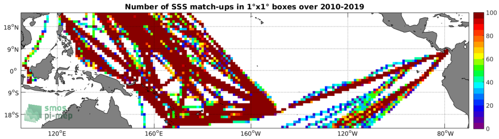
Figure 4: Number of SSS match-ups between TSG (LEGOS-DM) SSS and the SMOS SSS L3 v4 - 18 Days (CATDS-CECOS-LOCEAN) SSS product for the Tropical Pacific Ocean Pi-MEP region over 1^\circ \times 1^\circ boxes and for the full satellite product period.
