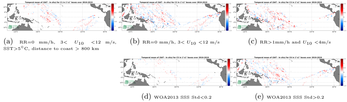
Figure 12: Temporal mean gridded over spatial boxes of size 1^{\circ}\times 1^{\circ} of \Delta\text{SSS} (SMOS-L3-CATDS-CECOS-LOCEAN-V4-18DAYS-25KM - TSG-LEGOS-DM) for 5 different subdatasets corresponding to: RR=0 mm/h, 3 < U_{10} < 12 m/s, SST > 5^{\circ}\text{C} , distance to coast > 800 km (a), RR=0 mm/h, 3 < U_{10} < 12 m/s (b), RR > 1 mm/h and U_{10} < 4 m/s (c), WOA2013 SSS Std < 0.2 (d), WOA2013 SSS Std > 0.2 (e).
