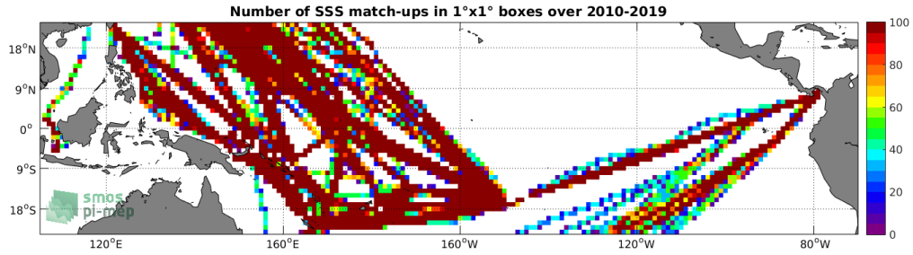
Figure 4: Number of SSS match-ups between TSG-LEGOS-DM SSS and the SMOS-L3-CATDS-CECOS-LOCEAN-V4-18DAYS-25KM SSS product for the Tropical Pacific Ocean Pi-MEP region over 1^\circ \times 1^\circ boxes and for the full satellite product period.
