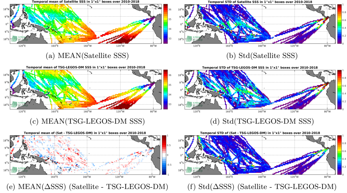
Figure 6: Temporal mean (left) and Std (right) of SSS from SMOS-L3-CATDS-CECOS-LOCEAN-V4-18DAYS-25KM (top), TSG-LEGOS-DM (middle), and of \Delta SSS (Satellite - TSG-LEGOS-DM). Only match-up pairs are used to generate these maps.
