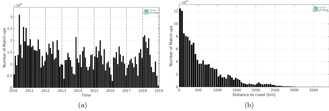
Figure 1: Number of match-ups between TSG-LEGOS-DM and SMOS-L3-CATDS-CECOS-LOCEAN-V4-18DAYS-25KM SSS as a function of time (a) and as function of the distance to coast (b) over the Tropical Pacific Ocean Pi-MEP region and for the full satellite product period.
