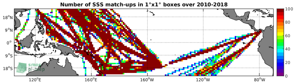
Figure 4: Number of SSS match-ups between TSG-LEGOS-DM SSS and the SMOS-L3-CATDS-CECOS-LOCEAN-V4-18DAYS-25KM SSS product for the Tropical Pacific Ocean Pi-MEP region over 1°x1° boxes and for the full satellite product period.
