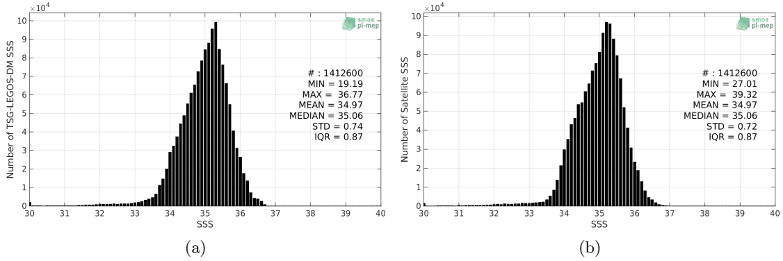
Figure 2: Histograms of SSS from TSG-LEGOS-DM (a) and SMOS-L3-CATDS-CECOS-LOCEAN-V4-18DAYS-25KM (b) considering all match-up pairs per bins of 0.1 over the Tropical Pacific Ocean Pi-MEP region and for the full satellite product period.
