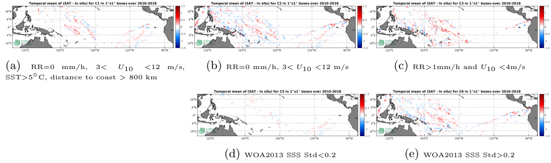
Figure 12: Temporal mean gridded over spatial boxes of size 1^\circ \times 1^\circ of \Delta SSS (SMOS-L3-CATDS-CECOS-LOCEAN-V4-18DAYS-25KM - TSG-LEGOS-DM) for 5 different subdatasets corresponding to: RR=0 mm/h, 3 < U_{10} < 12 m/s, SST > 5^\circ\text{C} , distance to coast > 800 km (a), RR=0 mm/h, 3 < U_{10} < 12 m/s (b), RR > 1 mm/h and U_{10} < 4 m/s (c), WOA2013 SSS Std < 0.2 (d), WOA2013 SSS Std > 0.2 (e).
