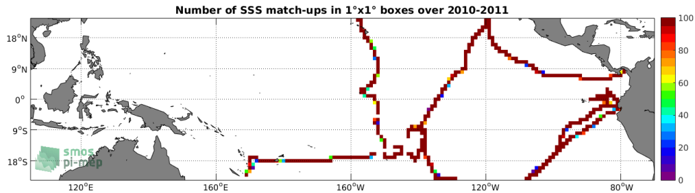
Figure 4: Number of SSS match-ups between TSG-GOSUD-Sailing-ship SSS and the SMOS-L3-CATDS-CECOS-LOCEAN-V4-18DAYS-25KM SSS product for the Tropical Pacific Ocean Pi-MEP region over 1^\circ \times 1^\circ boxes and for the full satellite product period.
