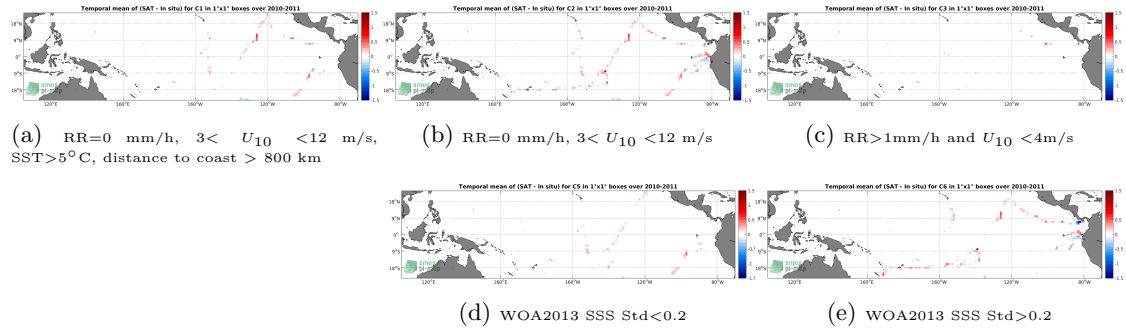
Figure 12: Temporal mean gridded over spatial boxes of size 1^{\circ}\times 1^{\circ} of \Delta SSS (SMOS-L3-CATDS-CECOS-LOCEAN-V4-18DAYS-25KM - TSG-GOSUD-Sailing-ship) for 5 different subdatasets corresponding to:RR=0 mm/h, 3 < U_{10} < 12 m/s, SST >5^{\circ}\text{C} , distance to coast > 800 km (a), RR=0 mm/h, 3 < U_{10} < 12 m/s (b), RR >1 mm/h and U_{10} < 4 m/s (c), WOA2013 SSS Std <0.2 (d), WOA2013 SSS Std >0.2 (e).
