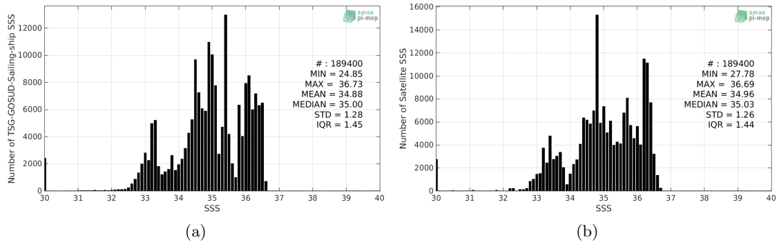
Figure 2: Histograms of SSS from TSG-GOSUD-Sailing-ship (a) and SMOS-L3-CATDS-CECOS-LOCEAN-V4-18DAYS-25KM (b) considering all match-up pairs per bins of 0.1 over the Tropical Pacific Ocean Pi-MEP region and for the full satellite product period.
