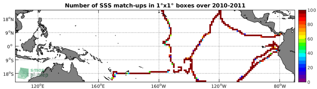
Figure 4: Number of SSS match-ups between TSG-GOSUD-Sailing-ship SSS and the SMOS-L3-CATDS-CECOS-LOCEAN-V4-18DAYS-25KM SSS product for the Tropical Pacific Ocean Pi-MEP region over 1^\circ \times 1^\circ boxes and for the full satellite product period.
