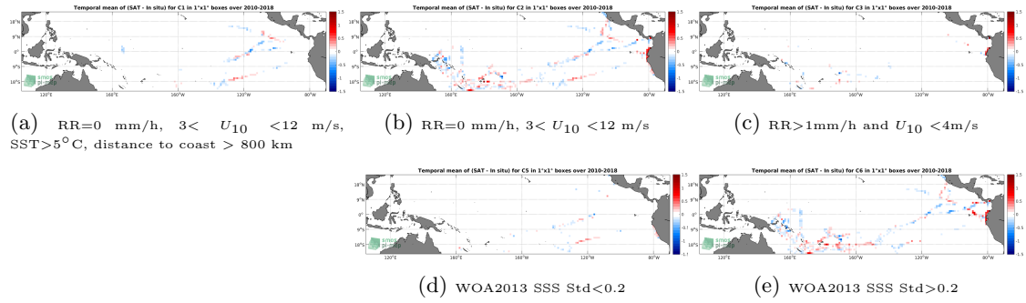
Figure 12: Temporal mean gridded over spatial boxes of size 1^\circ \times 1^\circ of \Delta SSS (SMOS SSS L3 v4 - 18 Days (CATDS-CECOS-LOCEAN) - TSG (GOSUD-Research-vessel)) for 5 different subdatasets corresponding to: RR=0 mm/h, 3 < U_{10} < 12 m/s, SST > 5^\circ\text{C} , distance to coast > 800 km (a), RR=0 mm/h, 3 < U_{10} < 12 m/s (b), RR > 1 mm/h and U_{10} < 4 m/s (c), WOA2013 SSS Std < 0.2 (d), WOA2013 SSS Std > 0.2 (e).
