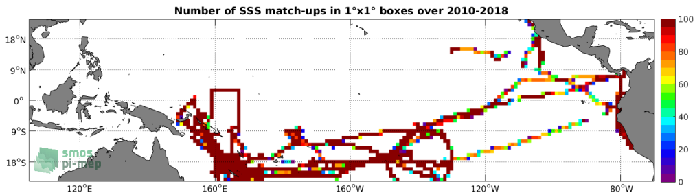
Figure 4: Number of SSS match-ups between TSG (GOSUD-Research-vessel) SSS and the SMOS SSS L3 v4 - 18 Days (CATDS-CECOS-LOCEAN) SSS product for the Tropical Pacific Ocean Pi-MEP region over 1^\circ \times 1^\circ boxes and for the full satellite product period.
