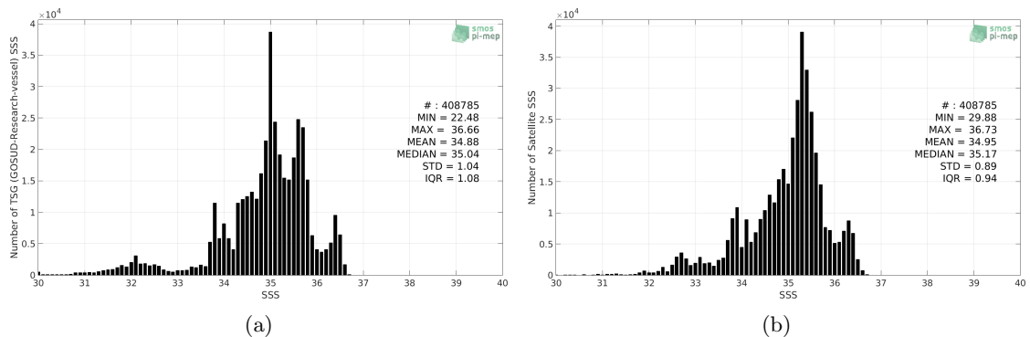
Figure 2: Histograms of SSS from TSG (GOSUD-Research-vessel) (a) and SMOS SSS L3 v4 - 18 Days (CATDS-CECOS-LOCEAN) (b) considering all match-up pairs per bins of 0.1 over the Tropical Pacific Ocean Pi-MEP region and for the full satellite product period.
