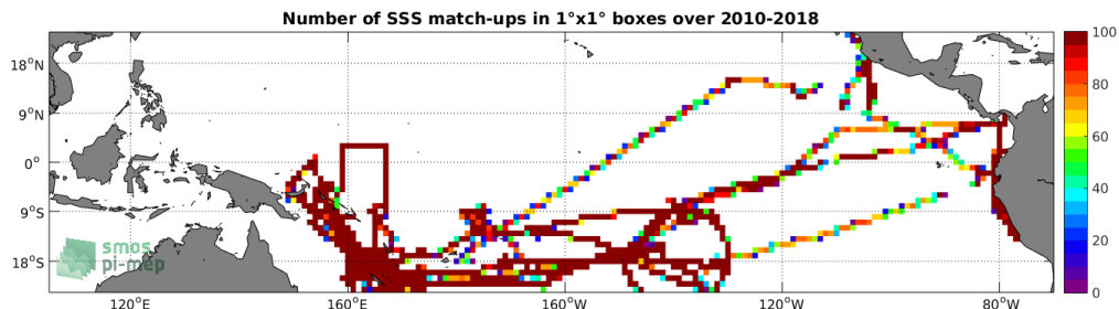
Figure 4: Number of SSS match-ups between TSG-GOSUD-Research-vessel SSS and the SMOS-L3-CATDS-CECOS-LOCEAN-V4-18DAYS-25KM SSS product for the Tropical Pacific Ocean Pi-MEP region over 1^\circ \times 1^\circ boxes and for the full satellite product period.
