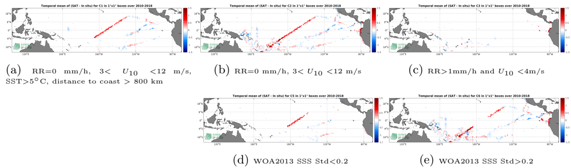
Figure 12: Temporal mean gridded over spatial boxes of size 1^{\circ}\times 1^{\circ} of \Delta SSS (SMOS-L3-CATDS-CECOS-LOCEAN-V4-18DAYS-25KM - TSG-GOSUD-Research-vessel) for 5 different subdatasets corresponding to:RR=0 mm/h, 3 < U_{10} < 12 m/s, SST >5^{\circ}\text{C} , distance to coast > 800 km (a), RR=0 mm/h, 3 < U_{10} < 12 m/s (b), RR >1 mm/h and U_{10} < 4 m/s (c), WOA2013 SSS Std <0.2 (d), WOA2013 SSS Std >0.2 (e).
