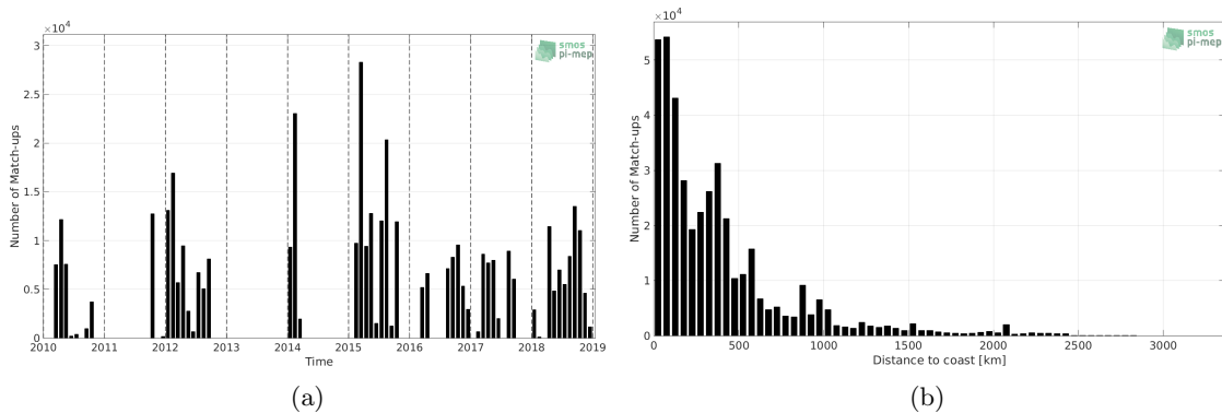
Figure 1: Number of match-ups between TSG-GOSUD-Research-vessel and SMOS-L3-CATDS-CECOS-LOCEAN-V4-18DAYS-25KM SSS as a function of time (a) and as function of the distance to coast (b) over the Tropical Pacific Ocean Pi-MEP region and for the full satellite product period.
