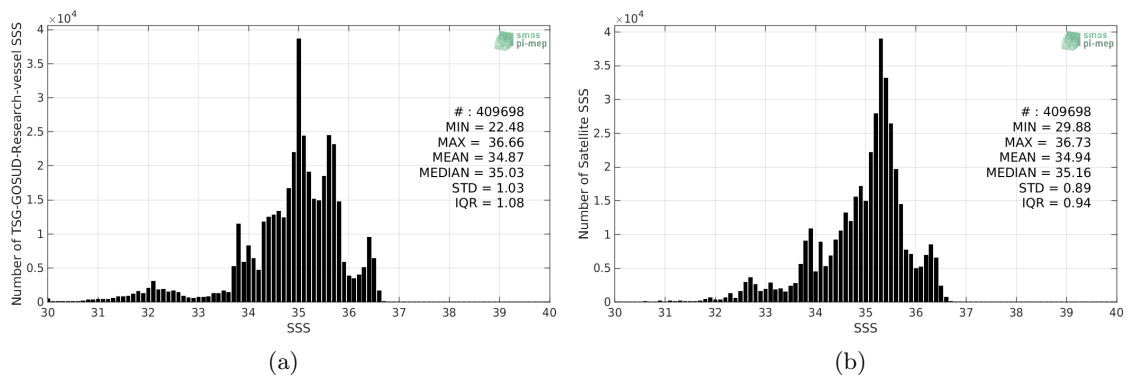
Figure 2: Histograms of SSS from TSG-GOSUD-Research-vessel (a) and SMOS-L3-CATDS-CECOS-LOCEAN-V4-18DAYS-25KM (b) considering all match-up pairs per bins of 0.1 over the Tropical Pacific Ocean Pi-MEP region and for the full satellite product period.
