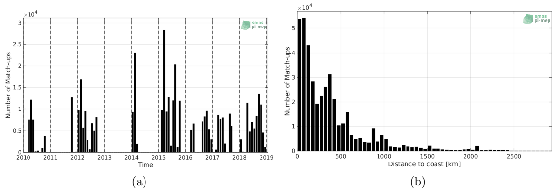
Figure 1: Number of match-ups between TSG-GOSUD-Research-vessel and SMOS-L3-CATDS-CECOS-LOCEAN-V4-18DAYS-25KM SSS as a function of time (a) and as function of the distance to coast (b) over the Tropical Pacific Ocean Pi-MEP region and for the full satellite product period.
