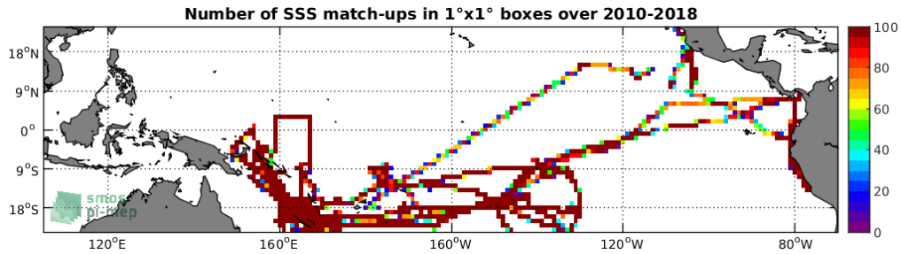
Figure 4: Number of SSS match-ups between TSG-GOSUD-Research-vessel SSS and the SMOS-L3-CATDS-CECOS-LOCEAN-V4-18DAYS-25KM SSS product for the Tropical Pacific Ocean Pi-MEP region over 1°x1° boxes and for the full satellite product period.
