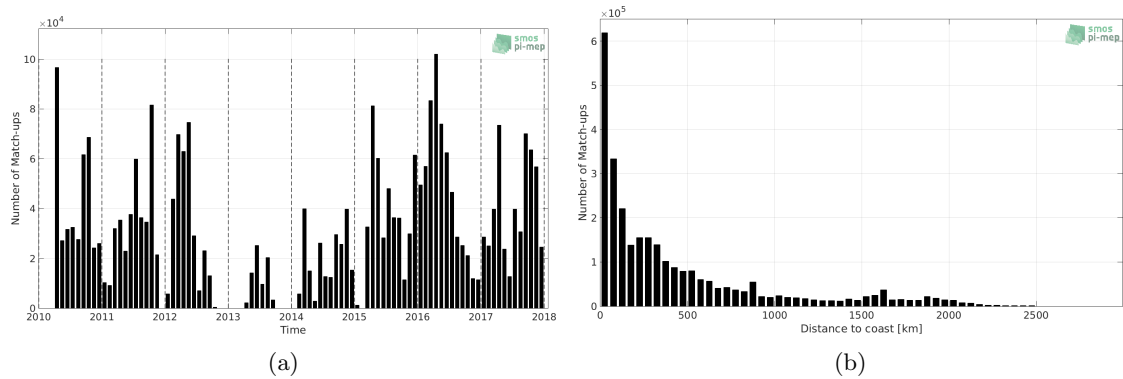
Figure 1: Number of match-ups between TSG-SAMOS and SMOS-L3-CATDS-CECOS-LOCEAN-V3-9DAYS-25KM SSS as a function of time (a) and as function of the distance to coast (b) over the Tropical Pacific Ocean Pi-MEP region and for the full satellite product period.
