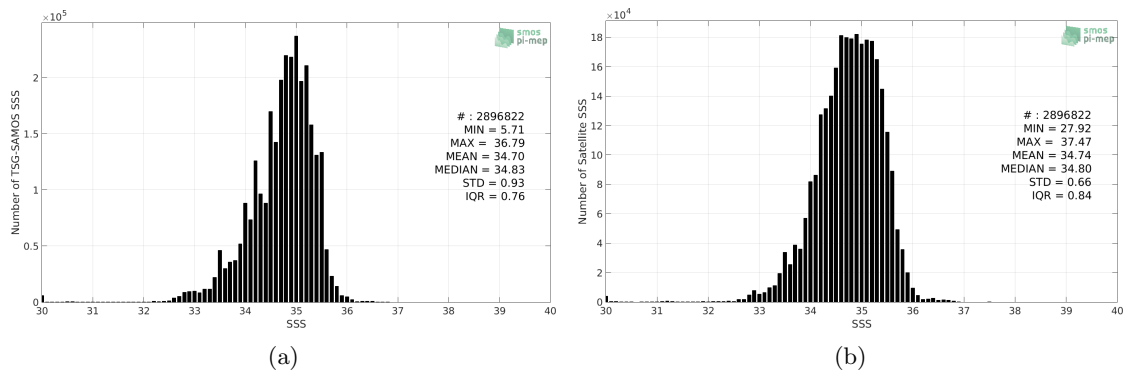
Figure 2: Histograms of SSS from TSG-SAMOS (a) and SMOS-L3-CATDS-CECOS-LOCEAN-V3-9DAYS-25KM (b) considering all match-up pairs per bins of 0.1 over the Tropical Pacific Ocean Pi-MEP region and for the full satellite product period.
