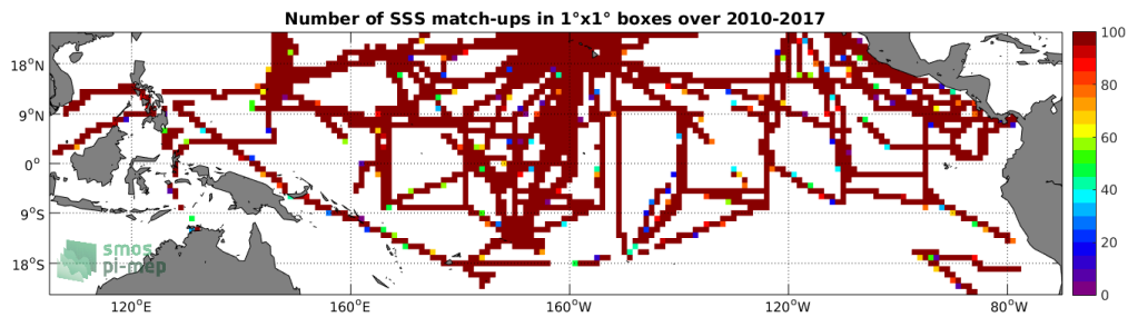
Figure 4: Number of SSS match-ups between TSG-SAMOS SSS and the SMOS-L3-CATDS-CECOS-LOCEAN-V3-9DAYS-25KM SSS product for the Tropical Pacific Ocean Pi-MEP region over 1^\circ \times 1^\circ boxes and for the full satellite product period.
