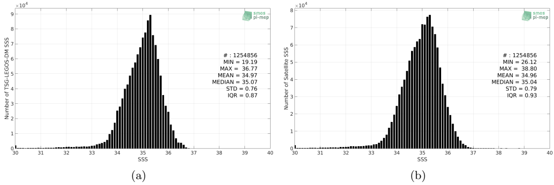
Figure 2: Histograms of SSS from TSG-LEGOS-DM (a) and SMOS-L3-CATDS-CECOS-LOCEAN-V3-9DAYS-25KM (b) considering all match-up pairs per bins of 0.1 over the Tropical Pacific Ocean Pi-MEP region and for the full satellite product period.
