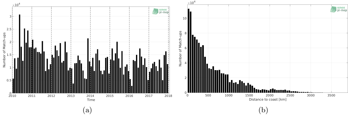
Figure 1: Number of match-ups between TSG-LEGOS-DM and SMOS-L3-CATDS-CECOS-LOCEAN-V3-9DAYS-25KM SSS as a function of time (a) and as function of the distance to coast (b) over the Tropical Pacific Ocean Pi-MEP region and for the full satellite product period.
