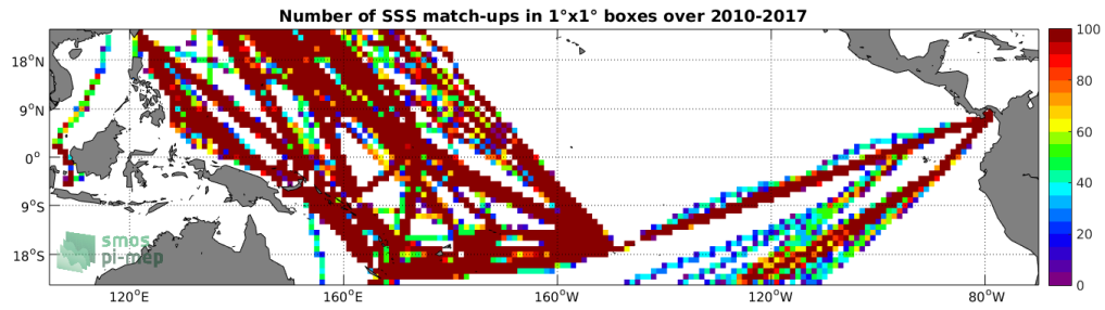
Figure 4: Number of SSS match-ups between TSG-LEGOS-DM SSS and the SMOS-L3-CATDS-CECOS-LOCEAN-V3-9DAYS-25KM SSS product for the Tropical Pacific Ocean Pi-MEP region over 1^\circ \times 1^\circ boxes and for the full satellite product period.
