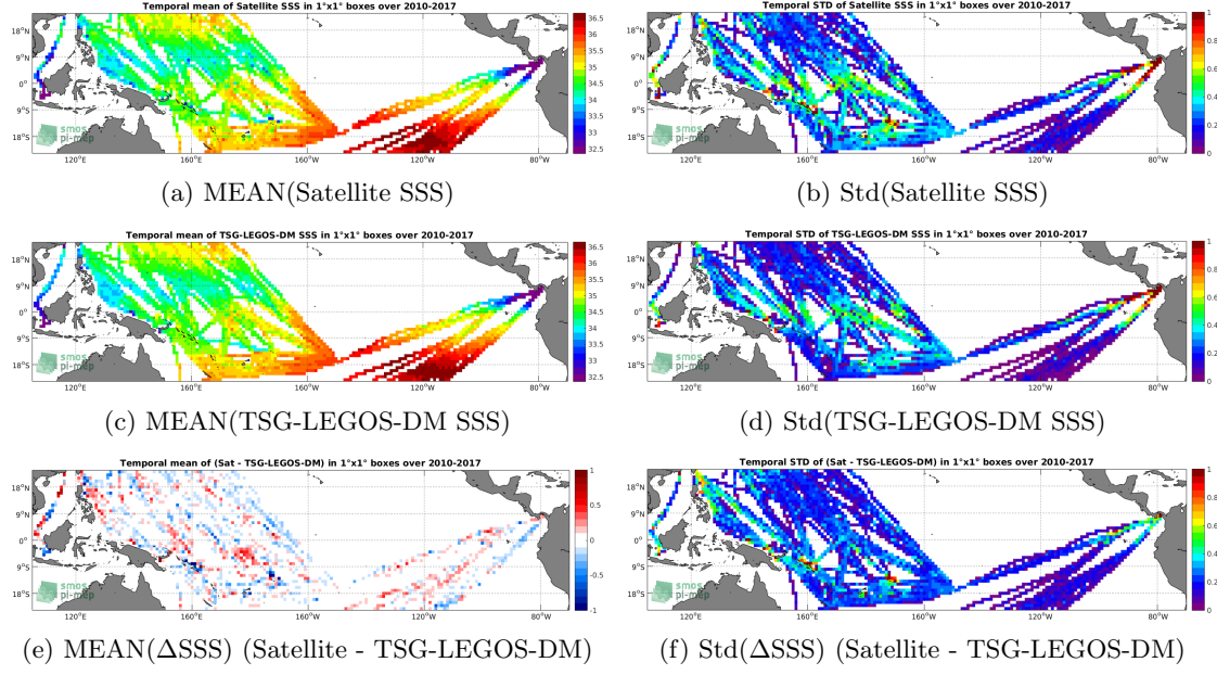
Figure 6: Temporal mean (left) and Std (right) of SSS from SMOS-L3-CATDS-CECOS-LOCEAN-V3-9DAYS-25KM (top), TSG-LEGOS-DM (middle), and of \Delta SSS (Satellite - TSG-LEGOS-DM). Only match-up pairs are used to generate these maps.
