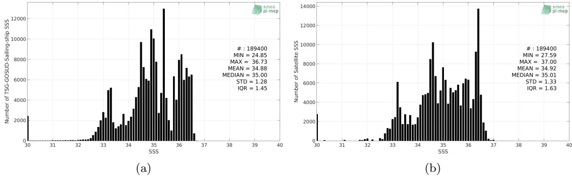
Figure 2: Histograms of SSS from TSG-GOSUD-Sailing-ship (a) and SMOS-L3-CATDS-CECOS-LOCEAN-V3-9DAYS-25KM (b) considering all match-up pairs per bins of 0.1 over the Tropical Pacific Ocean Pi-MEP region and for the full satellite product period.
