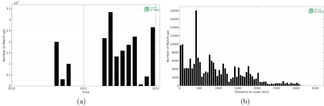
Figure 1: Number of match-ups between TSG-GOSUD-Sailing-ship and SMOS-L3-CATDS-CECOS-LOCEAN-V3-9DAYS-25KM SSS as a function of time (a) and as function of the distance to coast (b) over the Tropical Pacific Ocean Pi-MEP region and for the full satellite product period.
