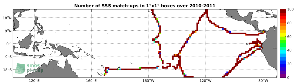
Figure 4: Number of SSS match-ups between TSG-GOSUD-Sailing-ship SSS and the SMOS-L3-CATDS-CECOS-LOCEAN-V3-9DAYS-25KM SSS product for the Tropical Pacific Ocean Pi-MEP region over 1^\circ \times 1^\circ boxes and for the full satellite product period.
