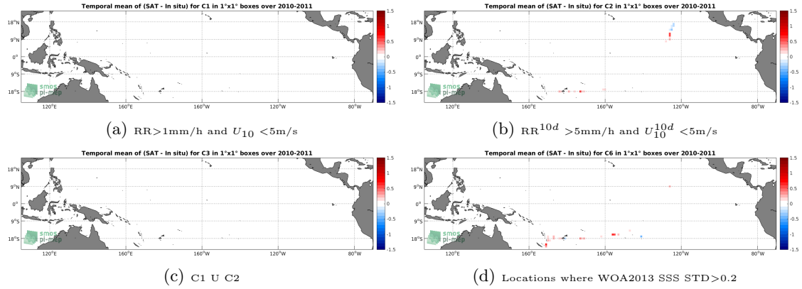
Figure 12: Temporal mean gridded over spatial boxes of size 1^\circ \times 1^\circ of \Delta SSS (SMOS-L3-CATDS-CECOS-LOCEAN-V3-9DAYS-25KM - TSG-GOSUD-Sailing-ship) for 4 different subdatasets corresponding to: RR > 1\text{mm/h} and U_{10} < 5\text{m/s} (a), RR^{10d} > 5\text{mm/h} and U_{10}^{10d} < 5\text{m/s} (b), C1 U C2 (c), Locations where WOA2013 SSS STD > 0.2 (d).
