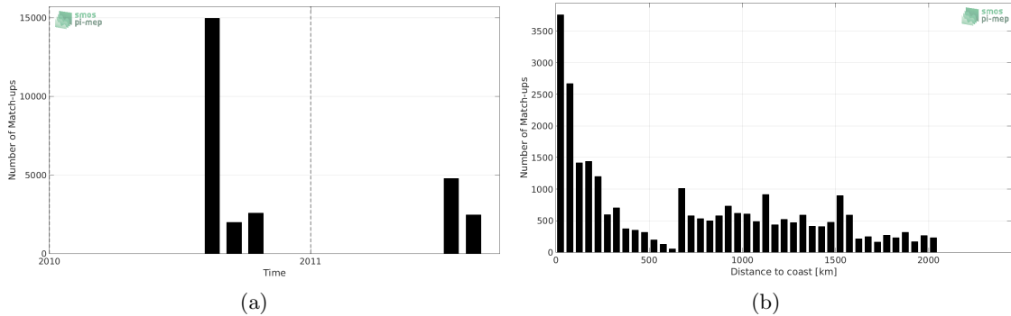
Figure 1: Number of match-ups between TSG-GOSUD-Sailing-ship and SMOS-L3-CATDS-CECOS-LOCEAN-V3-9DAYS-25KM SSS as a function of time (a) and as function of the distance to coast (b) over the Tropical Pacific Ocean Pi-MEP region and for the full satellite product period.
