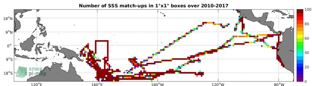
Figure 4: Number of SSS match-ups between TSG-GOSUD-Research-vessel SSS and the SMOS-L3-CATDS-CECOS-LOCEAN-V3-9DAYS-25KM SSS product for the Tropical Pacific Ocean Pi-MEP region over 1^\circ \times 1^\circ boxes and for the full satellite product period.
