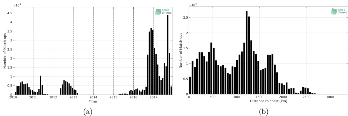
Figure 1: Number of match-ups between Surface drifters and SMOS-L3-CATDS-CECOS-LOCEAN-V3-9DAYS-25KM SSS as a function of time (a) and as function of the distance to coast (b) over the Tropical Pacific Ocean Pi-MEP region and for the full satellite product period.
