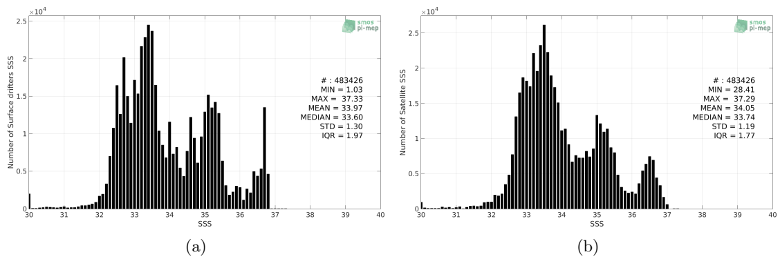
Figure 2: Histograms of SSS from Surface drifters (a) and SMOS-L3-CATDS-CECOS-LOCEAN-V3-9DAYS-25KM (b) considering all match-up pairs per bins of 0.1 over the Tropical Pacific Ocean Pi-MEP region and for the full satellite product period.
