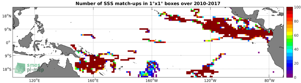
Figure 3: Number of SSS match-ups between Surface drifters SSS and the SMOS-L3-CATDS-CECOS-LOCEAN-V3-9DAYS-25KM SSS product for the Tropical Pacific Ocean Pi-MEP region over 1^\circ \times 1^\circ boxes and for the full satellite product period.
