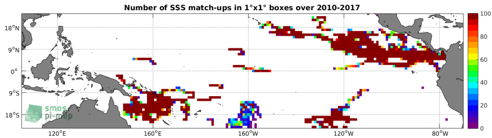
Figure 3: Number of SSS match-ups between Surface drifters SSS and the SMOS-L3-CATDS-CECOS-LOCEAN-V3-9DAYS-25KM SSS product for the Tropical Pacific Ocean Pi-MEP region over 1^\circ \times 1^\circ boxes and for the full satellite product period.
