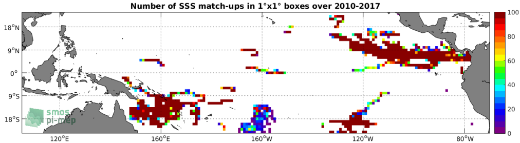
Figure 3: Number of SSS match-ups between Surface drifters SSS and the SMOS-L3-CATDS-CECOS-LOCEAN-V3-9DAYS-25KM SSS product for the Tropical Pacific Ocean Pi-MEP region over 1^{\circ} \times 1^{\circ} boxes and for the full satellite product period.
