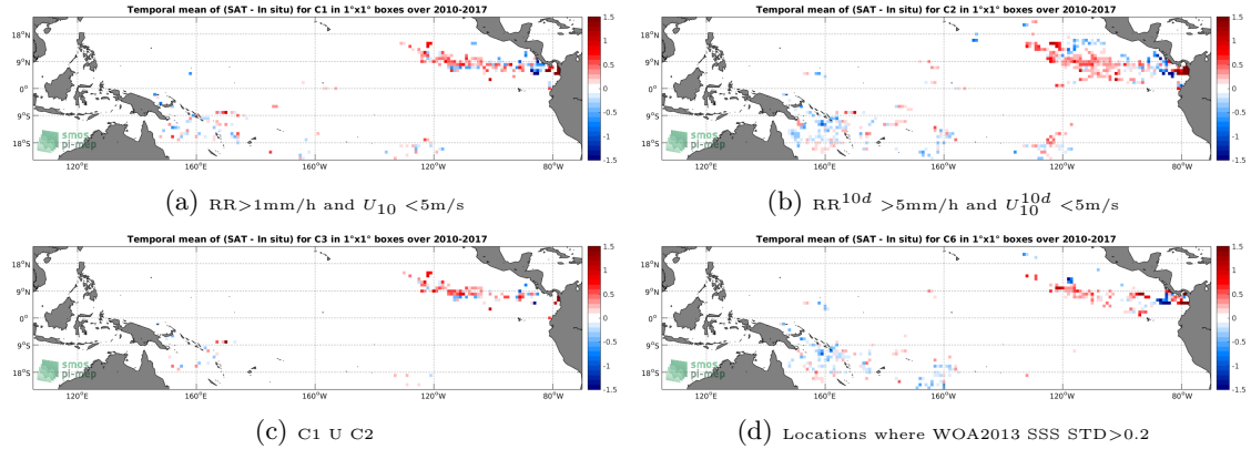
Figure 11: Temporal mean gridded over spatial boxes of size 1^\circ \times 1^\circ of \Delta SSS (SMOS-L3-CATDS-CECOS-LOCEAN-V3-9DAYS-25KM - Surface drifters) for 4 different subdatasets corresponding to: RR > 1\text{mm/h} and U_{10} < 5\text{m/s} (a), RR^{10d} > 5\text{mm/h} and U_{10}^{10d} < 5\text{m/s} (b), C1 U C2 (c), Locations where WOA2013 SSS STD > 0.2 (d).
