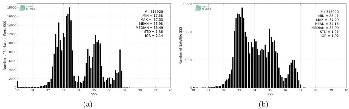
Figure 2: Histograms of SSS from Surface drifters (a) and SMOS-L3-CATDS-CECOS-LOCEAN-V3-9DAYS-25KM (b) considering all match-up pairs per bins of 0.1 over the Tropical Pacific Ocean Pi-MEP region and for the full satellite product period.
