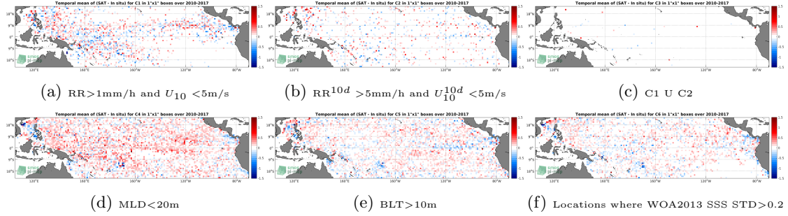
Figure 12: Temporal mean gridded over spatial boxes of size 1^\circ \times 1^\circ of \Delta SSS (SMOS-L3-CATDS-CECOS-LOCEAN-V3-9DAYS-25KM - Argo) for 6 different subdatasets corresponding to:RR>1mm/h and U_{10} < 5\text{m/s} (a), RR^{10d} > 5\text{mm/h} and U_{10}^{10d} < 5\text{m/s} (b), C1 U C2 (c),MLD<20m (d),BLT>10m (e),Locations where WOA2013 SSS STD>0.2 (f).
