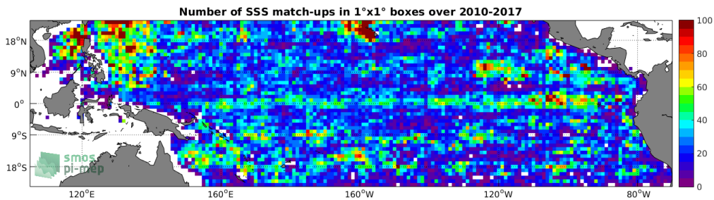
Figure 4: Number of SSS match-ups between Argo SSS and the SMOS-L3-CATDS-CECOS-LOCEAN-V3-9DAYS-25KM SSS product for the Tropical Pacific Ocean Pi-MEP region over 1^\circ \times 1^\circ boxes and for the full satellite product period.
