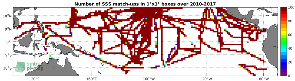
Figure 4: Number of SSS match-ups between TSG-SAMOS SSS and the SMOS-L3-CATDS-CECOS-LOCEAN-V3-18DAYS-25KM SSS product for the Tropical Pacific Ocean Pi-MEP region over 1^\circ \times 1^\circ boxes and for the full satellite product period.
