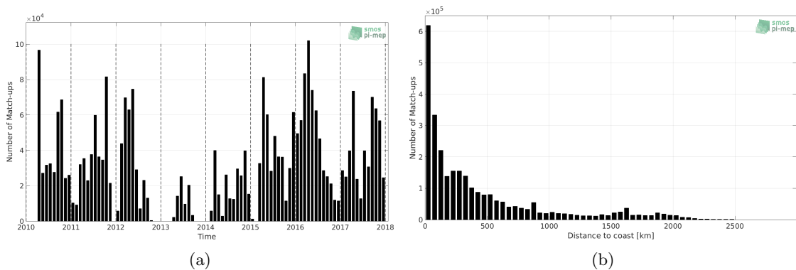
Figure 1: Number of match-ups between TSG-SAMOS and SMOS-L3-CATDS-CECOS-LOCEAN-V3-18DAYS-25KM SSS as a function of time (a) and as function of the distance to coast (b) over the Tropical Pacific Ocean Pi-MEP region and for the full satellite product period.
