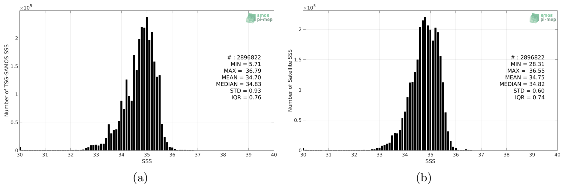
Figure 2: Histograms of SSS from TSG-SAMOS (a) and SMOS-L3-CATDS-CECOS-LOCEAN-V3-18DAYS-25KM (b) considering all match-up pairs per bins of 0.1 over the Tropical Pacific Ocean Pi-MEP region and for the full satellite product period.
