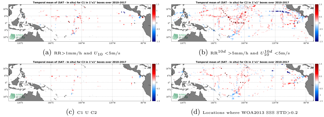
Figure 12: Temporal mean gridded over spatial boxes of size 1^\circ \times 1^\circ of \Delta SSS (SMOS-L3-CATDS-CECOS-LOCEAN-V3-18DAYS-25KM - TSG-SAMOS) for 4 different subdatasets corresponding to: RR > 1 mm/h and U_{10} < 5 m/s (a), RR 10d > 5 mm/h and U_{10}^{10d} < 5 m/s (b), C1 U C2 (c), Locations where WOA2013 SSS STD > 0.2 (d).
