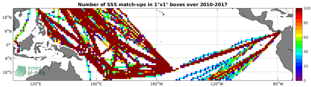
Figure 4: Number of SSS match-ups between TSG-LEGOS-DM SSS and the SMOS-L3-CATDS-CECOS-LOCEAN-V3-18DAYS-25KM SSS product for the Tropical Pacific Ocean Pi-MEP region over 1^\circ \times 1^\circ boxes and for the full satellite product period.
