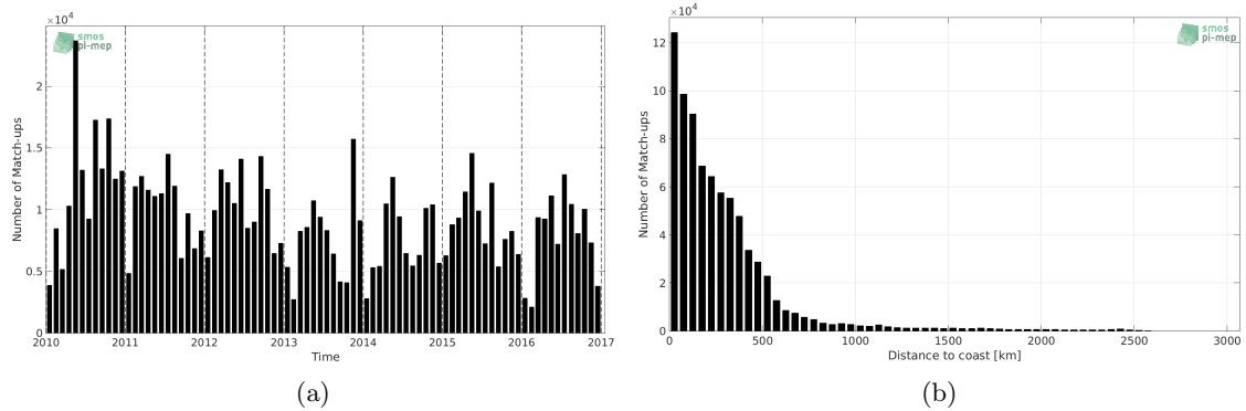
Figure 1: Number of match-ups between TSG-LEGOS-DM and SMOS-L3-CATDS-CECOS-LOCEAN-V3-18DAYS-25KM SSS as a function of time (a) and as function of the distance to coast (b) over the Tropical Pacific Ocean Pi-MEP region and for the full satellite product period.
