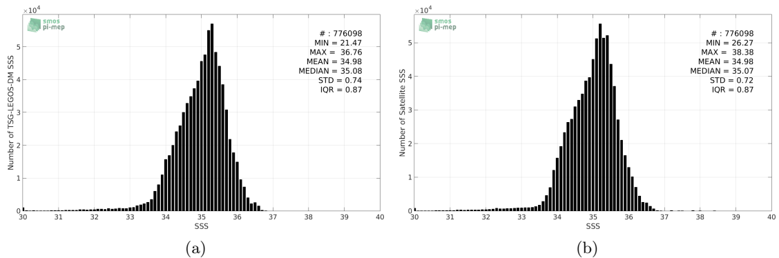
Figure 2: Histograms of SSS from TSG-LEGOS-DM (a) and SMOS-L3-CATDS-CECOS-LOCEAN-V3-18DAYS-25KM (b) considering all match-up pairs per bins of 0.1 over the Tropical Pacific Ocean Pi-MEP region and for the full satellite product period.
