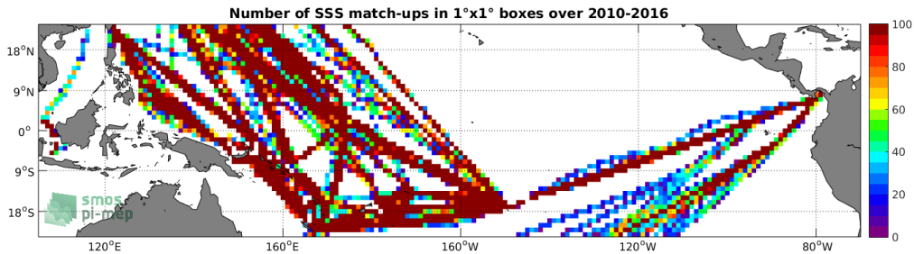
Figure 4: Number of SSS match-ups between TSG-LEGOS-DM SSS and the SMOS-L3-CATDS-CECOS-LOCEAN-V3-18DAYS-25KM SSS product for the Tropical Pacific Ocean Pi-MEP region over 1^\circ \times 1^\circ boxes and for the full satellite product period.
