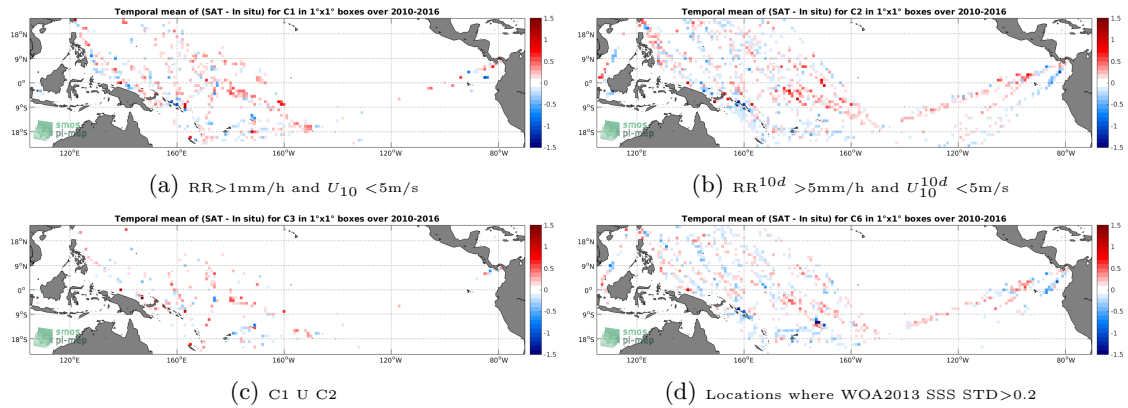
Figure 12: Temporal mean gridded over spatial boxes of size 1^\circ \times 1^\circ of \Delta SSS (SMOS-L3-CATDS-CECOS-LOCEAN-V3-18DAYS-25KM - TSG-LEGOS-DM) for 4 different subdatasets corresponding to: RR > 1mm/h and U_{10} < 5\text{m/s} (a), RR^{10d} > 5\text{mm/h} and U_{10}^{10d} < 5\text{m/s} (b), C1 U C2 (c), Locations where WOA2013 SSS STD > 0.2 (d).
