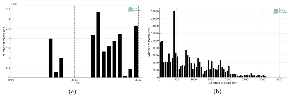
Figure 1: Number of match-ups between TSG-GOSUD-Sailing-ship and SMOS-L3-CATDS-CECOS-LOCEAN-V3-18DAYS-25KM SSS as a function of time (a) and as function of the distance to coast (b) over the Tropical Pacific Ocean Pi-MEP region and for the full satellite product period.
