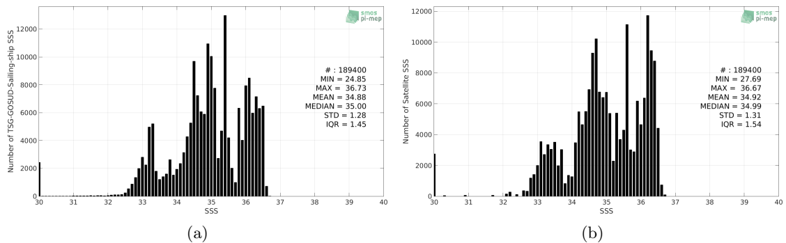
Figure 2: Histograms of SSS from TSG-GOSUD-Sailing-ship (a) and SMOS-L3-CATDS-CECOS-LOCEAN-V3-18DAYS-25KM (b) considering all match-up pairs per bins of 0.1 over the Tropical Pacific Ocean Pi-MEP region and for the full satellite product period.
