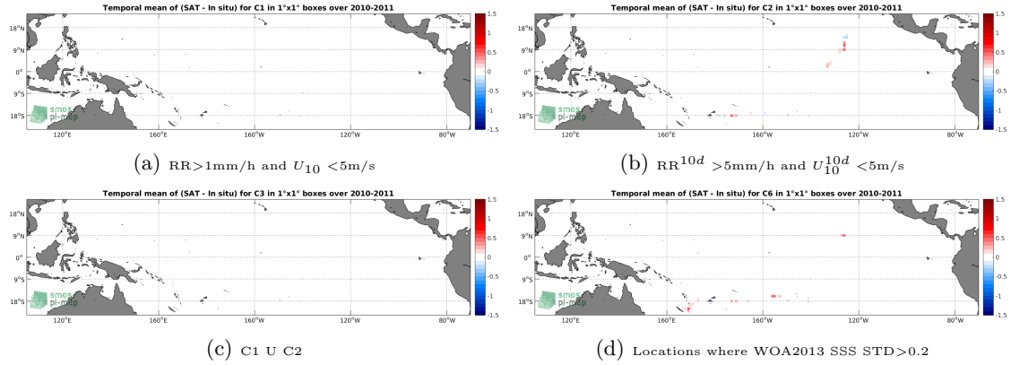
Figure 12: Temporal mean gridded over spatial boxes of size 1^\circ \times 1^\circ of \Delta SSS (SMOS-L3-CATDS-CECOS-LOCEAN-V3-18DAYS-25KM - TSG-GOSUD-Sailing-ship) for 4 different subdatasets corresponding to: RR > 1mm/h and U_{10} < 5\text{m/s} (a), RR^{10d} > 5\text{mm/h} and U_{10}^{10d} < 5\text{m/s} (b), C1 U C2 (c), Locations where WOA2013 SSS STD > 0.2 (d).
