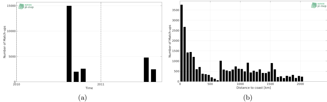
Figure 1: Number of match-ups between TSG-GOSUD-Sailing-ship and SMOS-L3-CATDS-CECOS-LOCEAN-V3-18DAYS-25KM SSS as a function of time (a) and as function of the distance to coast (b) over the Tropical Pacific Ocean Pi-MEP region and for the full satellite product period.
