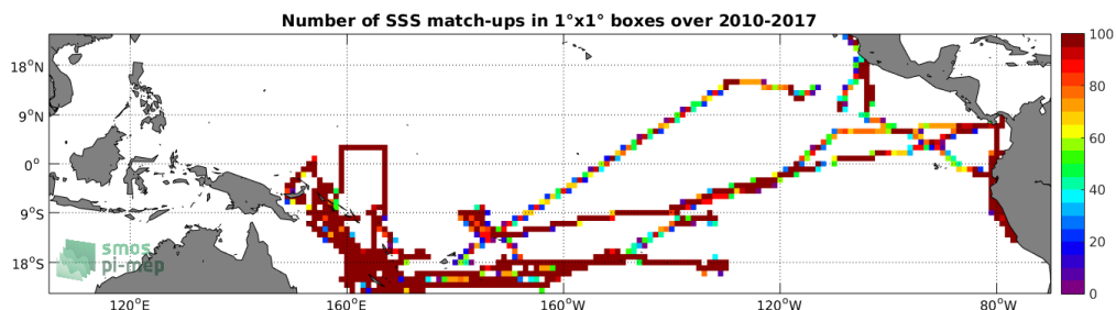
Figure 4: Number of SSS match-ups between TSG-GOSUD-Research-vessel SSS and the SMOS-L3-CATDS-CECOS-LOCEAN-V3-18DAYS-25KM SSS product for the Tropical Pacific Ocean Pi-MEP region over 1^\circ \times 1^\circ boxes and for the full satellite product period.
