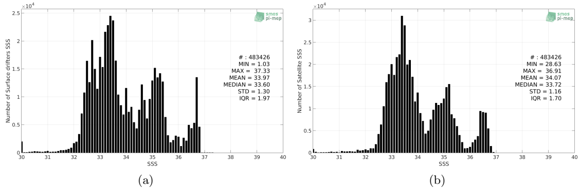
Figure 2: Histograms of SSS from Surface drifters (a) and SMOS-L3-CATDS-CECOS-LOCEAN-V3-18DAYS-25KM (b) considering all match-up pairs per bins of 0.1 over the Tropical Pacific Ocean Pi-MEP region and for the full satellite product period.
