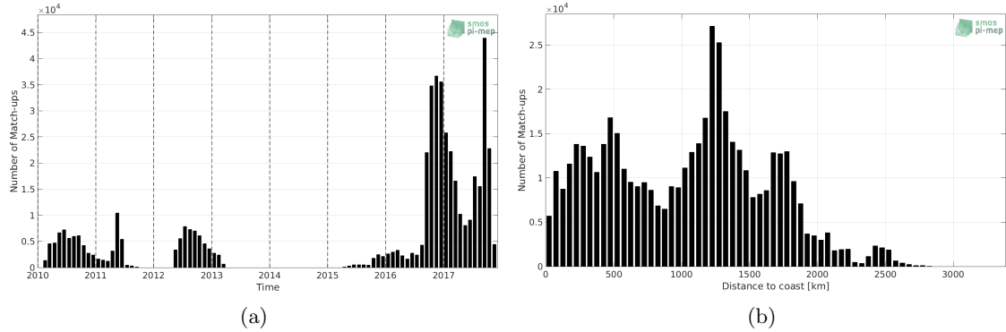
Figure 1: Number of match-ups between Surface drifters and SMOS-L3-CATDS-CECOS-LOCEAN-V3-18DAYS-25KM SSS as a function of time (a) and as function of the distance to coast (b) over the Tropical Pacific Ocean Pi-MEP region and for the full satellite product period.
