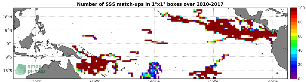
Figure 3: Number of SSS match-ups between Surface drifters SSS and the SMOS-L3-CATDS-CECOS-LOCEAN-V3-18DAYS-25KM SSS product for the Tropical Pacific Ocean Pi-MEP region over 1^\circ \times 1^\circ boxes and for the full satellite product period.
