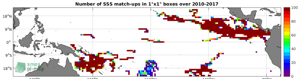
Figure 3: Number of SSS match-ups between Surface drifters SSS and the SMOS-L3-CATDS-CECOS-LOCEAN-V3-18DAYS-25KM SSS product for the Tropical Pacific Ocean Pi-MEP region over 1°x1° boxes and for the full satellite product period.
